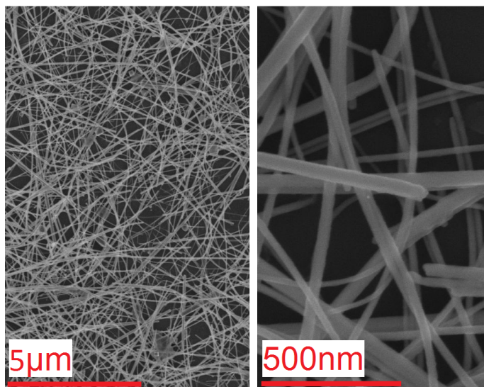
Fig. 1 Network-forming nature of long and thin CuNWs (approximately 27.6 nm in diameter, 62.36 \mu\text{m} long, and possessing an aspect ratio of 2200 on average). A vast number of connections that is a result of annealing can be seen while a large area for light to penetrate is maintained.
