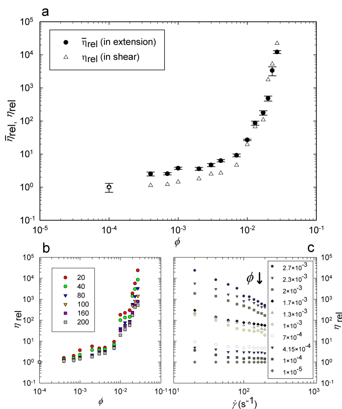
Fig. 3 (a) Relative extensional \bar{\eta}_{rel} and shear viscosity \eta_{rel} showing similar behavioural trends as a function of the volume fraction \phi . The shear viscosity values correspond to comparable extensional and shear strain rates. It should be noted that Sec.3.2 describes how the extensional viscosities seen here were extracted. (b) Relative shear viscosity against volume fraction for shear rates \dot{\gamma} of 20, 40, 80, 160, and 200 s^{-1} . (c) Relative shear viscosity against shear rate for different volume fractions, displaying pronounced shear thinning.
