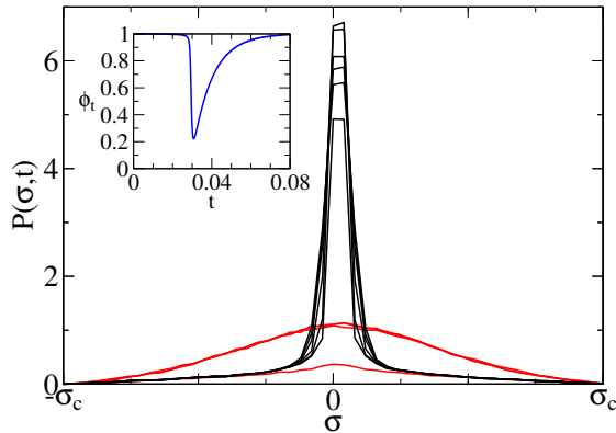
FIG. 3: Empirical distribution of stress variables \sigma_i for a population of N = 10^5 elements with zero shear rate. Different lines are relative to different snapshots taken at equally spaced time intervals of duration 0.01 (the corresponding value for the fraction of jammed elements as a function of time is plotted in the inset). Red lines correspond to the build up of the instability (the lower line is at t = 0.03 for example, approximately corresponding to the minimum of \phi(t) in the inset) while black lines correspond to elements progressively relaxing at \sigma = 0 . For illustrative purposes we set here \hat{\gamma} = 0 while other parameters are: \alpha = 1 , \tau_{fl} = 0.01 , D_i = 0.01 , dt = 10^{-6} , \hat{\omega} = 30 and \tau_{pl} = 0 .
