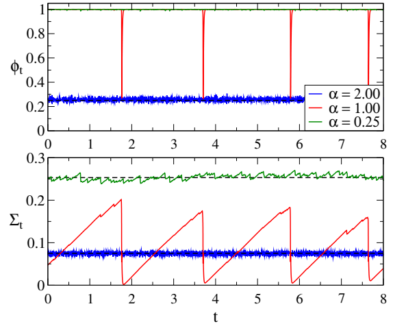
FIG. 2: Top : Fraction of jammed elements versus time for a population of N = 10^4 elements undergoing the random walk process described by Eq. (1) (see details in the text). Bottom : corresponding total stress as defined in Eq. (3). Different colors correspond to different values of the coupling constant \alpha (black dashed lines correspond to the analytical stationary solutions in the stable phase). Other parameters are: \hat{\gamma} = 0.001 , \hat{\omega} = 15 , D_i = 10^{-3} , dt = 10^{-6} and \tau_{\text{pl}} = 0 .
