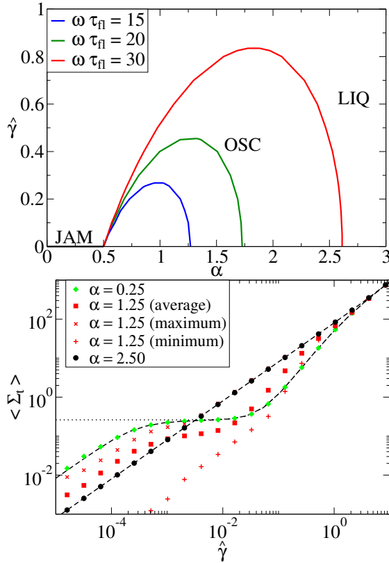
FIG. 1: Top : Phase diagram of the model in the (\alpha, \hat{\gamma}) plane (recall that \hat{\gamma} = \dot{\gamma}\tau_{fl} ) obtained from the solutions of Eq. (44) with D_i \rightarrow 0 and different values of \hat{\omega} = \omega\tau_{fl} . In the liquid (LIQ) phase, the system is stationary, and the flow curve is basically Newtonian in the whole range of \hat{\gamma} . In the jammed (JAM) phase, the system has a finite yield stress for \hat{\gamma} \rightarrow 0 . Finally, in the oscillating (OSC) phase, the stress is an oscillating function of time. Bottom : Flow curves displaying the average stress versus strain for \hat{\omega} = 20 , D_{int} = 0.005 , and three different values of \alpha corresponding to the jammed, oscillating, and liquid phases. Points correspond to numerical results while lines correspond to analytical results for the stationary state. For \alpha = 2.5 the system is liquid and the flow curve is Newtonian in all the regimes of \hat{\gamma} . For \alpha = 0.25 the system is jammed for \hat{\gamma} \rightarrow 0 and the stress tends to a finite value (dotted line), but in the simulation due to finite D_{int} we also see a Newtonian regime at small \hat{\gamma} (points and dashed line). For \alpha = 1.25 the system is oscillating for small \hat{\gamma} : in this case we report the minimum, average and maximum value of the stress (see Fig. 2 for an example).
