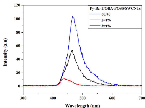
Figure 13 Fluorescence spectra of Py-Bz-T/OBA-POSS/SWCNT hybrid complexes
