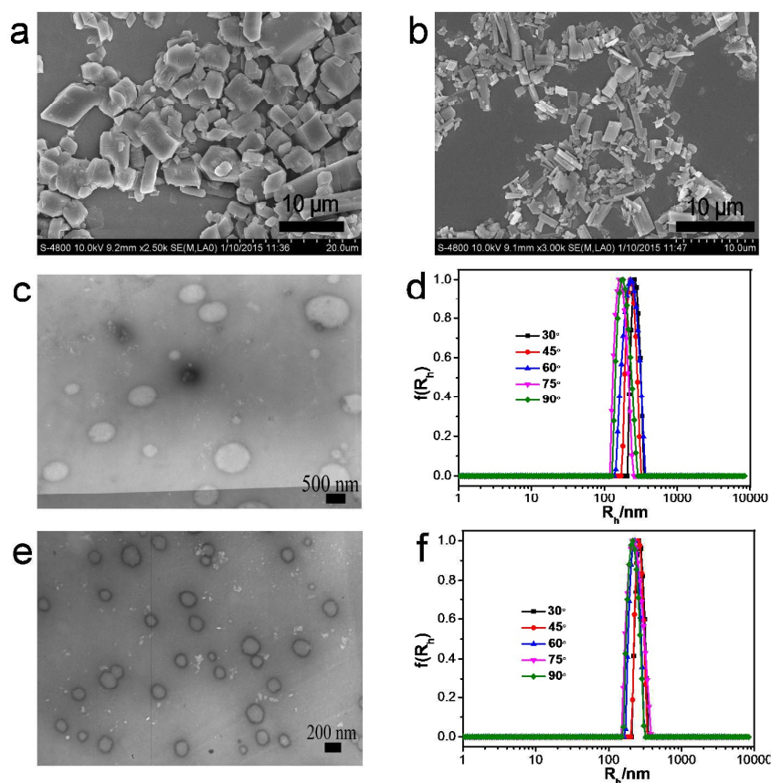
Figure 1. SEM micrographs of a) hexane/ \beta -CD precipitates and b) octadecane/ \beta -CD precipitates. TEM micrograph of c) the hexane/ \beta -CD sample ( C_{\text{hexane}@\beta\text{-CD}}=2 mM) and e) octadecane/ \beta -CD sample ( C_{\text{octadecane}@\beta\text{-CD}}=2 mM). DLS results at varying scattering angles of d) the hexane/ \beta -CD ( C_{\text{hexane}@\beta\text{-CD}}=2 mM) and f) octadecane/ \beta -CD sample ( C_{\text{octadecane}@\beta\text{-CD}}=2 mM).
