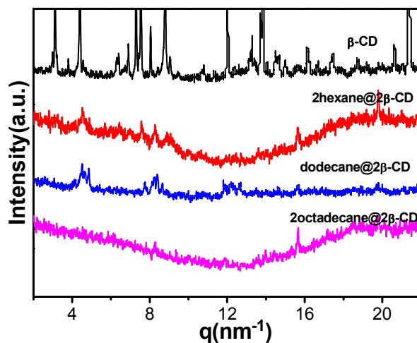
Figure 3. The SAXS spectrum of \beta -CD power and the lyophilized alkane (hexane, dodecane, octadecane)/ \beta -CD precipitates.
