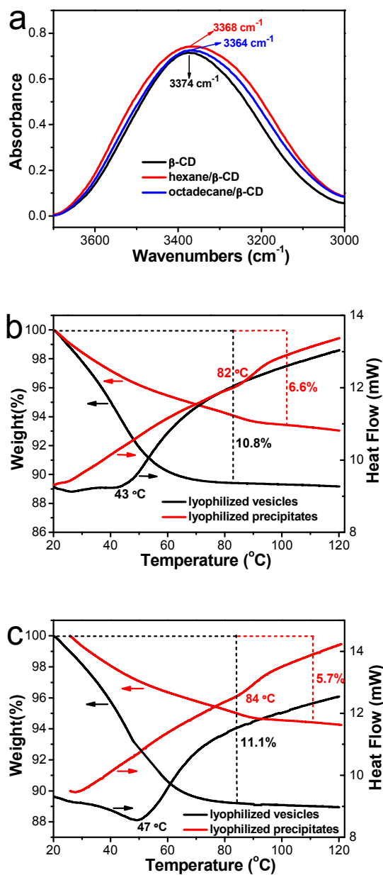
Figure 4. a) FT-IR spectra of \beta -CD power, the lyophilized hexane/ \beta -CD vesicles and octadecane/ \beta -CD vesicles. b) and c) TGA and DSC results of the lyophilized hexane/ \beta -CD and octadecane/ \beta -CD samples, respectively.
