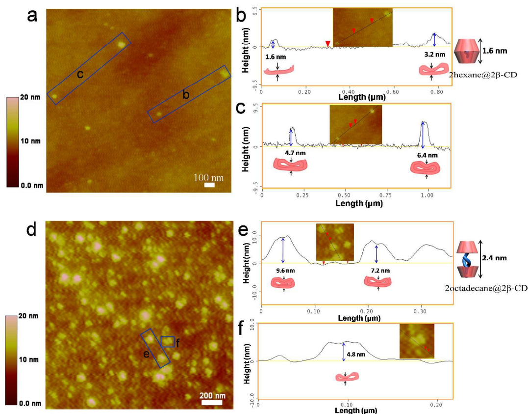
Figure 2. Images acquired by AFM for vesicles of a) hexane/ \beta -CD ( C_{\text{hexane}@\beta\text{-CD}}=2 mM) and d) octadecane/ \beta -CD ( C_{\text{octadecane}@\beta\text{-CD}}=2 mM) sample. b) and c) are the sectional height profiles of a collapsed unilamellar/bilamellar vesicle and the corresponding broken ones in a. e) and f) are the sectional height profiles of vesicles in d). The drawings in b) and e) are the illustrations of the supramolecular building blocks for 2\text{hexane}@2\beta\text{-CD} and 2\text{octadecane}@2\beta\text{-CD} , respectively.
