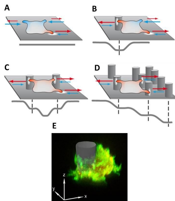
Figure 5: Schematic illustration of cell behaviour on different substrates, characterised by protrusion spreading (red) and retraction (blue), where extracellular obstacles can be described as potential wells promoting cellular motion processes; the resulting potential level is displayed in grey: (A) Random protrusion formation on flat substrates, (B) Protrusion stabilisation and subsequent adhesion to the additional surface contact with 3D structures, (C) Dynamic cell trapping effect by adhesion to multiple 3D structures in absence of other structures in the cell vicinity, (D) Topographic guidance effect by a gradual increase of the adhesion surface, (E) Fluorescent microscopy image of a D. discoideum cell expressing Lim-RFP and Arp2/3-GFP while adhering to a pillar structure
