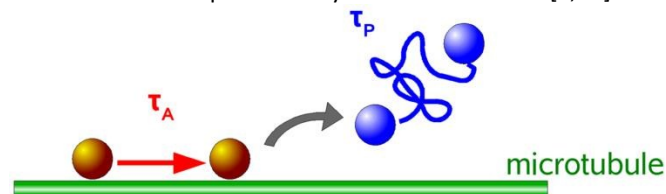
Figure 2: Two state distribution of tracer bead motion: State 1 – molecular motor associated motion along microtubules with attachment duration \tau_A . State 2 – detachment from microtubule and diffusive motion of duration \tau_P .
