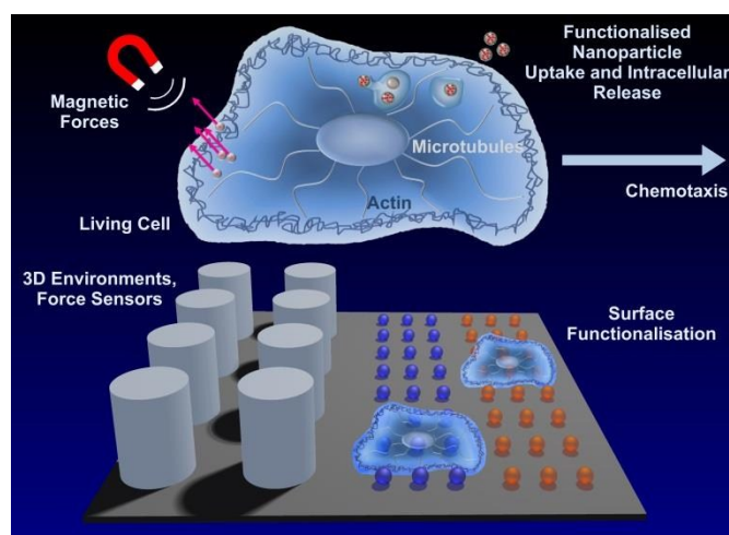
Figure 1: Schematic overview of experimental approaches for the elucidation of cell behaviour, signal processing and cell-substrate interaction. Intracellular information and material transport features are probed by uptake and intracellular release of functionalised nanoparticles in addition to magnetic force application. Cell-substrate interactions are investigated and will subsequently be controlled by cell type specific surface functionalisation. 3D environments are investigated and specifically adapted to match individual cell requirements for scaffold design. In addition force sensors for measurements of cell pulling and pushing forces are introduced.
