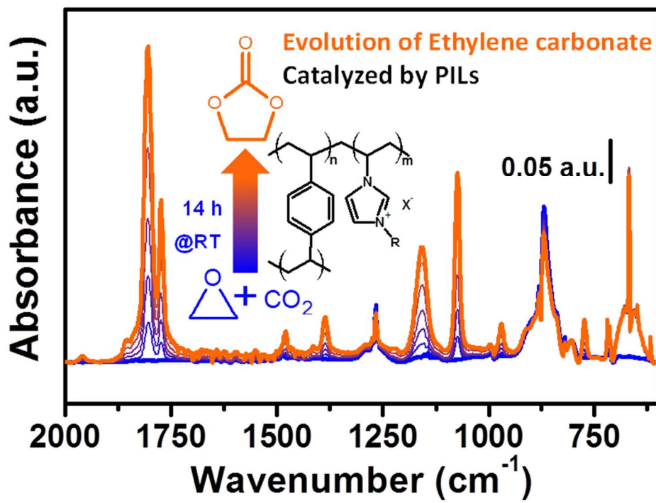
In situ FTIR monitoring the evolution of ethylene carbonate catalyzed by a designed high surface area poly(Ionic Liquid) 230x179mm (96 x 96 DPI)
