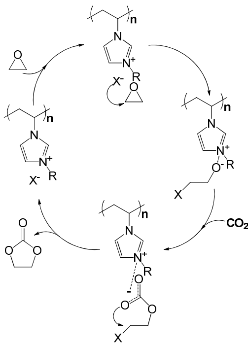
Scheme 3. Proposed scheme of the catalytic steps which occur in the reaction between carbon dioxide and ethylene oxide to produce ethylene carbonate over a PIL catalyst.
