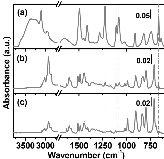
Figure 1. IR-ATR spectra of poly(VIm) (part a); co-polymer 1 (part b) and poly(DVB) (part c). Vertical lines evidence the position of the absorption bands which are the fingerprints of the imidazole ring.
