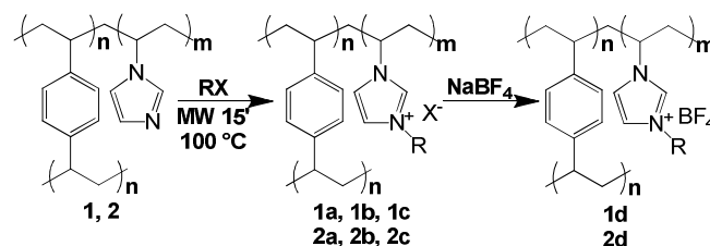
Scheme 2. Synthetic pathway for the PILs used in this work
