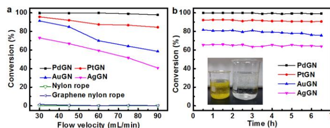
Fig. 5 Catalytic activity and stability of noble metal/graphene/nylon rope catalysts for reduction of 4-nitrophenol in the continuous-flow reactor. (a) Catalytic tests of the reduction rate for the reduction of 4-nitrophenol with different noble metal/graphene/nylon ropes at different flow velocities. (b) Catalytic stability: plots of conversion of 4-nitrophenol catalyzed by different noble metal/graphene/nylon ropes with a usage time of 6.5 hours. Inset shows the color change indicating the reduction of 4-nitrophenol to 4-aminophenol.
