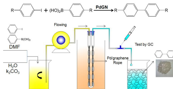
Fig. 2 Schematic representation for the continuous-flow system of Suzuki–Miyaura cross-coupling reactions catalyzed by Pd/graphene/nylon rope. The reaction is performed in a mixture solvent of DMF and water with a volume ratio of 1:1 at 90^\circ\text{C} at various flow rates.
