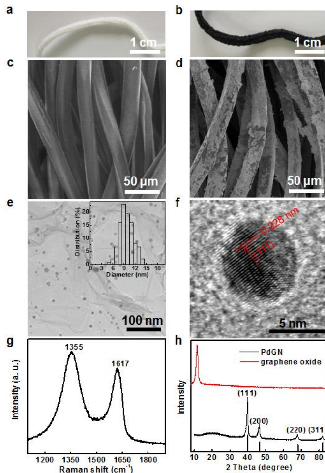
Fig. 1 Structural characterization of the PdGN catalysts. (a) Optical image of clean nylon rope. (b) Optical image of as-synthesized PdGN catalysts. (c) SEM image of clean nylon rope. (d) SEM image of PdGN catalysts. (e) TEM and (f) HRTEM images of Pd nanoparticles anchored on graphene obtained from 30 min ultrasonication of PdGN catalysts in ethanol. Inset is the size distribution of Pd nanoparticles loaded on PdGN catalysts. (g) Raman spectrum of PdGN catalysts. (h) XRD patterns of PdGN catalysts and graphene oxides.
