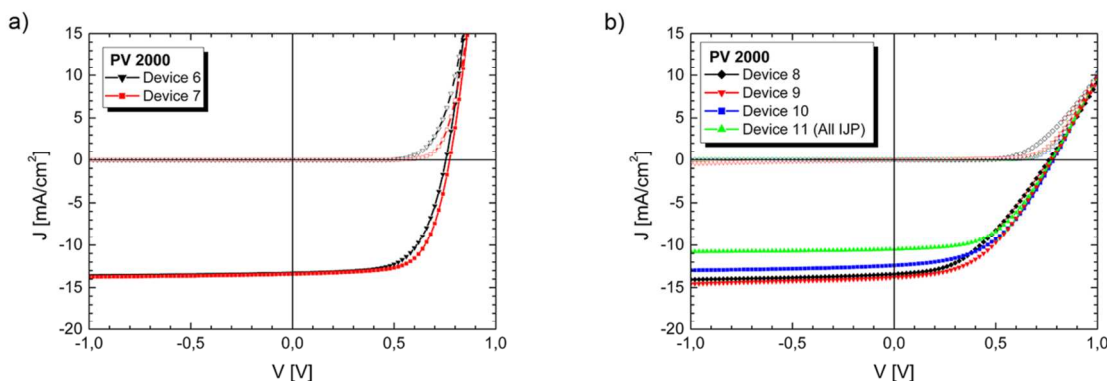
Figure 4. J-V curves recorded for inverted OPV cells with inkjet printed PV2000 photo-active layers and a) 0.038\text{ cm}^2 active area and evaporated back electrode, and b) 1\text{ cm}^2 active area and up to 6 inkjet printed layers.
