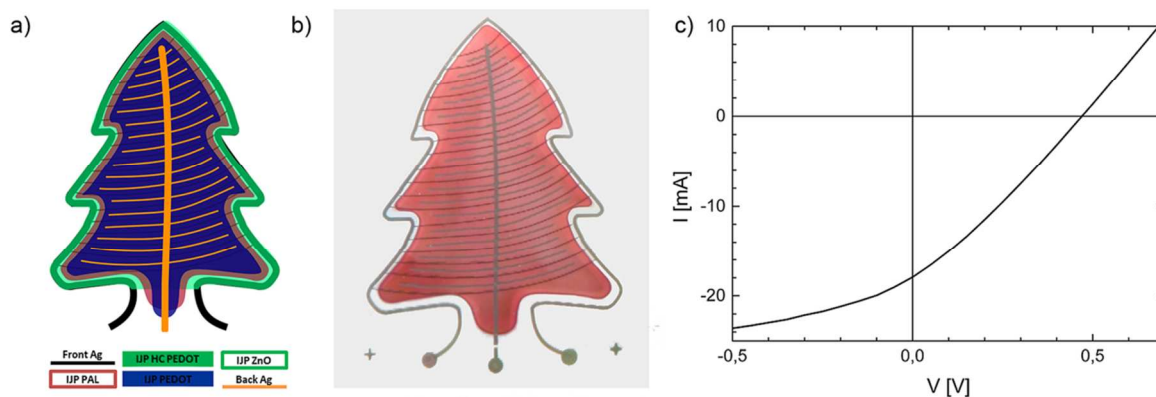
Figure 5. Organic solar cell in the shape of a Christmas tree, a) schematic representation of printed layers lay-out, b) photograph of finished fully inkjet printed OPV Christmas tree, and c) I-V curve recorded for a single device with Christmas tree shape.
