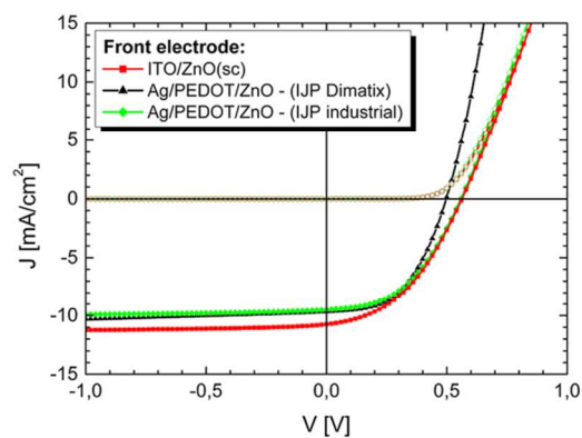
Figure 2. J-V curves recorded for devices with a spin coated P3HT:PCBM photo-active layer and an ITO front electrode or an inkjet printed electrode consisting of IJP Ag/IJP HC PEDOT/IJP ZnO (the active area of the devices is 0.038 \text{ cm}^2 ).
