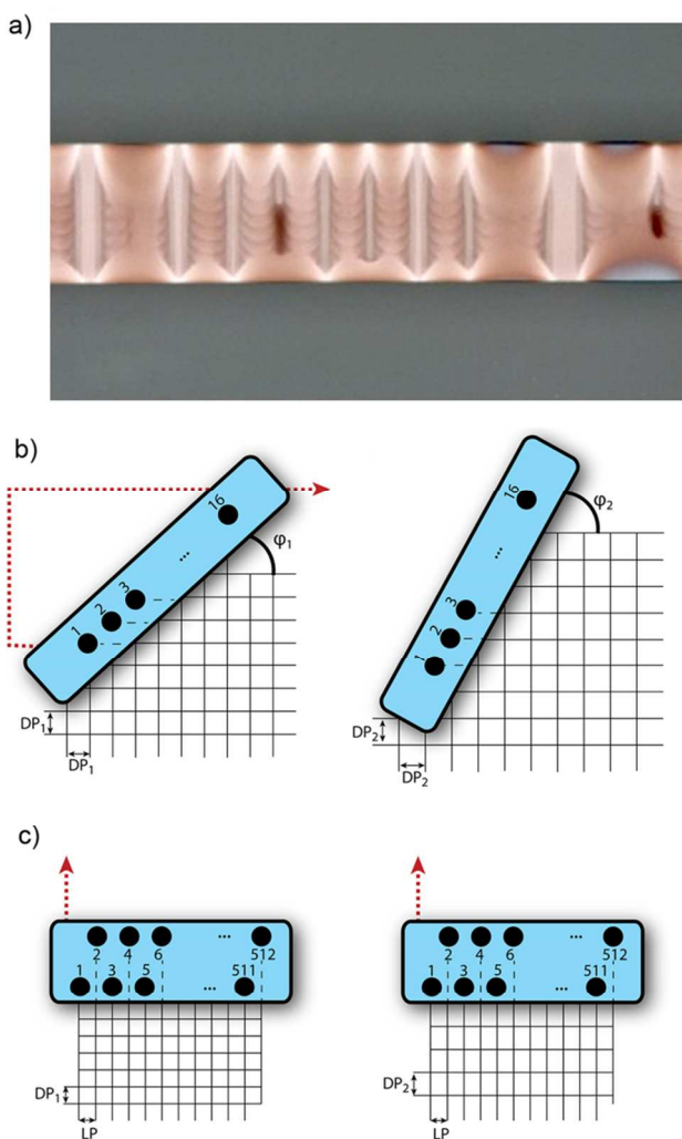
Figure 1. a) Optical microscopy image showing inhomogeneous coverage of HC-PEDOT printed on top of a Ag finger, b) printing mechanism with Dimatix printheads, c) printing mechanism with industrial printheads (arrows shows a printing direction).
