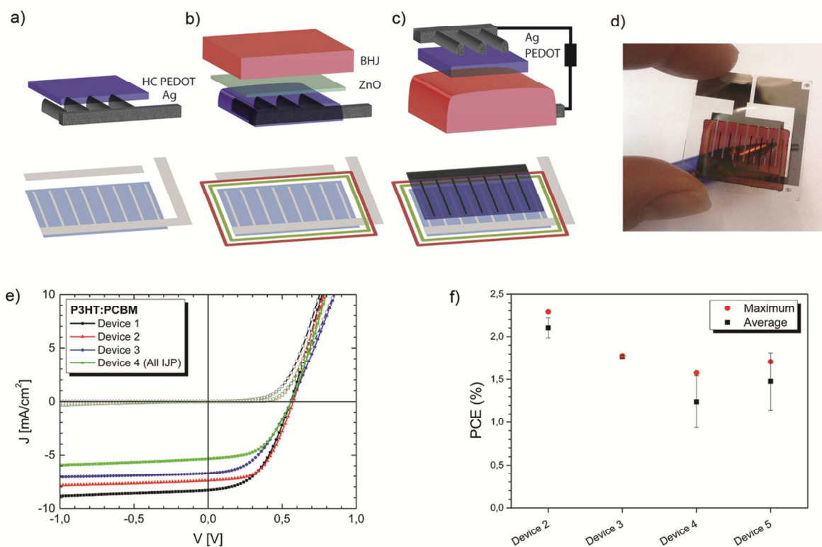
Figure 3. a-c) schematic representation of the layers in a fully inkjet printed organic solar cell, d) photograph of semitransparent all inkjet printed cell, by an illumination mask a 1 cm 2 active area is defined, e) J-V curves of cells with a P3HT:PCBM photo-active layer and multiple printed layers f) maximum and average performances (back electrode is: * - Ag grids, ** - full area Ag).
