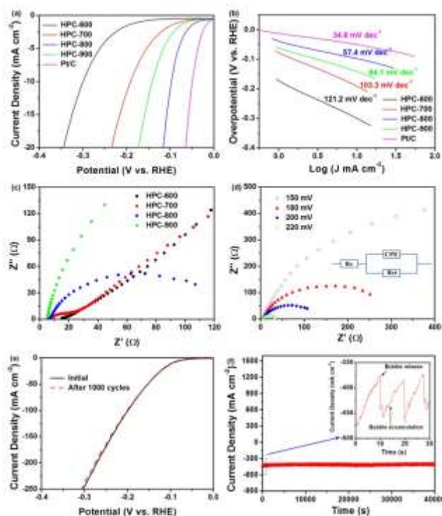
Figure 5. (a) HER polarization curves and (b) the corresponding Tafel plots of HPC-600, HPC-700, HPC-800, HPC-900, and Pt/C, at a potential scan rate of 5 mV s -1 in 0.5 M H 2 SO 4 . (c) Electrochemical impedance spectra of the various porous carbons in HER at –0.20 V (vs. RHE). (d) Electrochemical impedance spectra of HPC-800 at various overpotentials (specified in figure legends) for HER in 0.5 M H 2 SO 4 . Inset shows the equivalent circuit where R s is the (uncompensated) electrode series resistance, CPE is the constant-phase element and R ct is the charge-transfer resistance. (e) HER polarization curves for HPC-800 before and after 1000 cycles in the stability test. (f) Time dependence of the HER current density of HPC-800 at –0.15 V vs. RHE, where inset shows the impacts of bubbles formed on the electrode surface on the HER currents.
