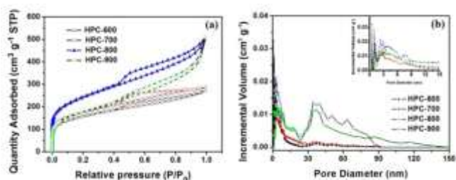
Figure 3. (a) N_2 adsorption-desorption isotherms and (b) pore-size distributions of HPC-600, HPC-700, HPC-800 and HPC-900. The inset to panel (b) is the zoom-in of the pore-size distributions at pore diameters lower than 15 nm.
