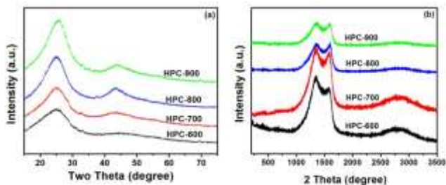
Figure 2. (a) XRD patterns and (b) Raman spectra of HPC-600, HPC-700, HPC-800 and HPC-900.
