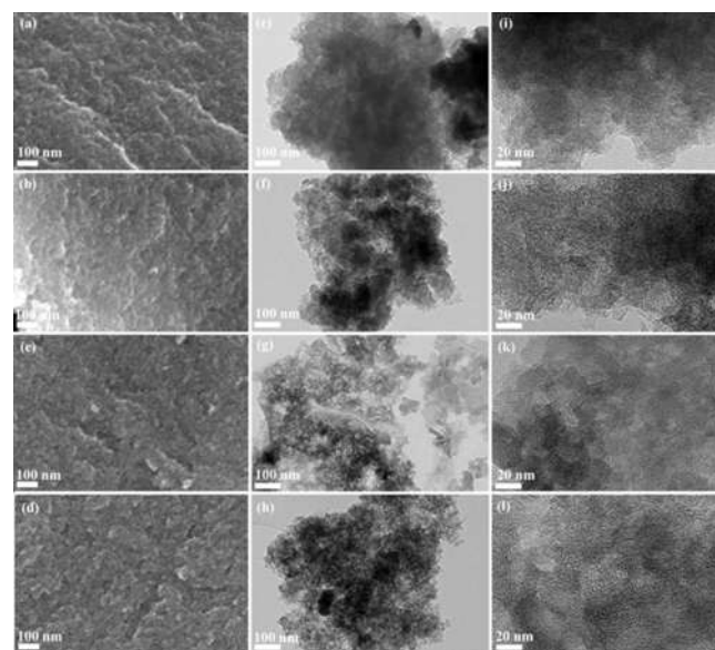
Figure 1. Representative SEM and TEM images of (a, e, i) HPC-600, (b, f, j) HPC-700, (c, g, k) HPC-800, and (d, h, l) HPC-900. Scale bars are 100 nm in panels (a) to (h) and 20 nm in panels (i) to (l).
