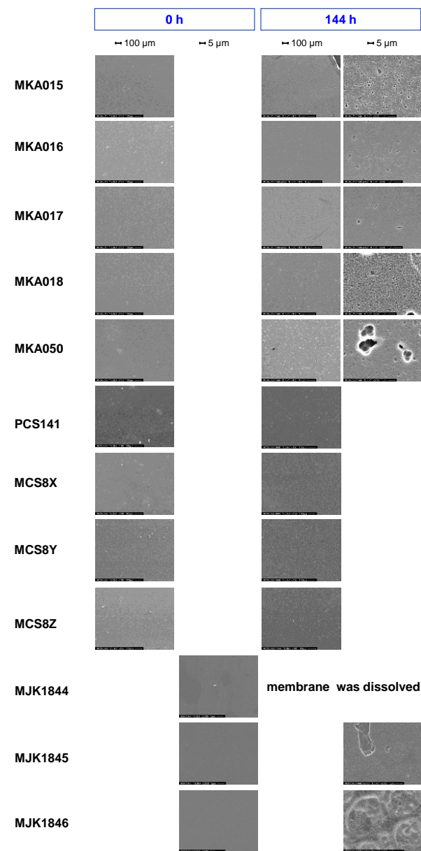
Fig. 8 SEM images of the membranes before and after 144 hours Fenton Test; magnification 100x/2000x.
