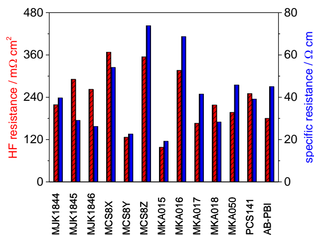
Fig. 11 High frequency resistance and specific resistance of the membranes; T=160\text{ }^{\circ}\text{C} , A=2.56\text{ cm}^2 , 1\text{ mg Pt cm}^{-2} , hydrogen/air with \lambda=1.4/2 , j=200\text{ mA cm}^{-2} .
