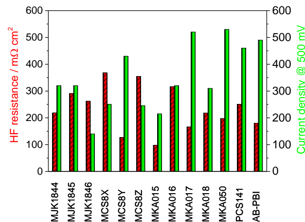
Fig. 13 High frequency resistance of the membranes and current density of the MEAs at 500\text{ mV} ; T = 160\text{ }^{\circ}\text{C} , A = 2.56\text{ cm}^2 , 1\text{ mg Pt cm}^{-2} , hydrogen/air with \lambda = 1.4/2 .
