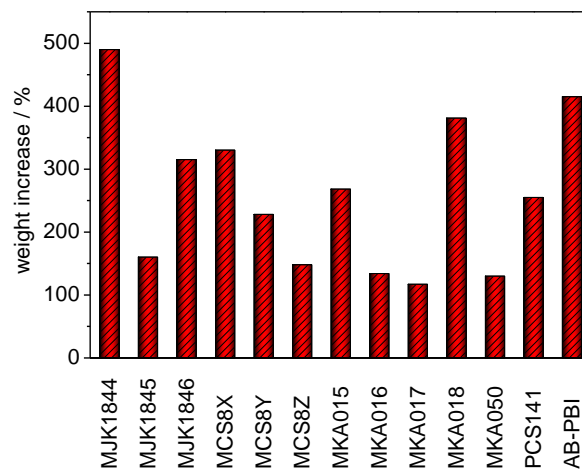
Fig. 9 Phosphoric acid uptake of the membranes by weight; T=130 °C (120 °C for AB-PBI).
