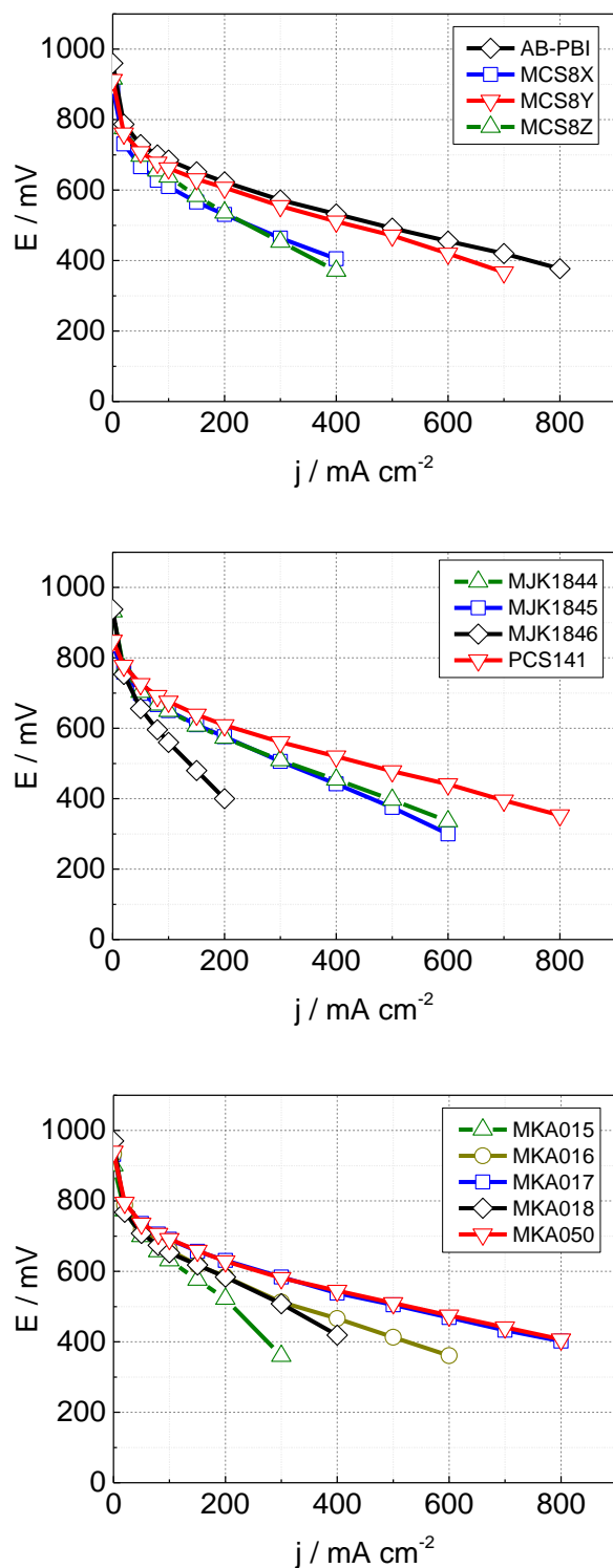
Fig. 12 Cell performance of MEAs with different membranes; T = 160\text{ }^{\circ}\text{C} , A = 4\text{ cm}^2 , 1\text{ mg Pt cm}^{-2} , \lambda (hydrogen) = 1.4, \lambda (air) = 2, ambient pressure.
