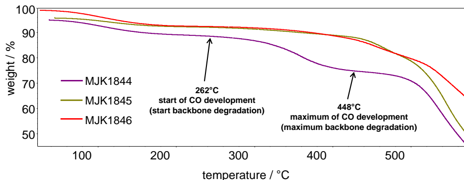
Fig. 4 TGA traces of the MJK membranes
