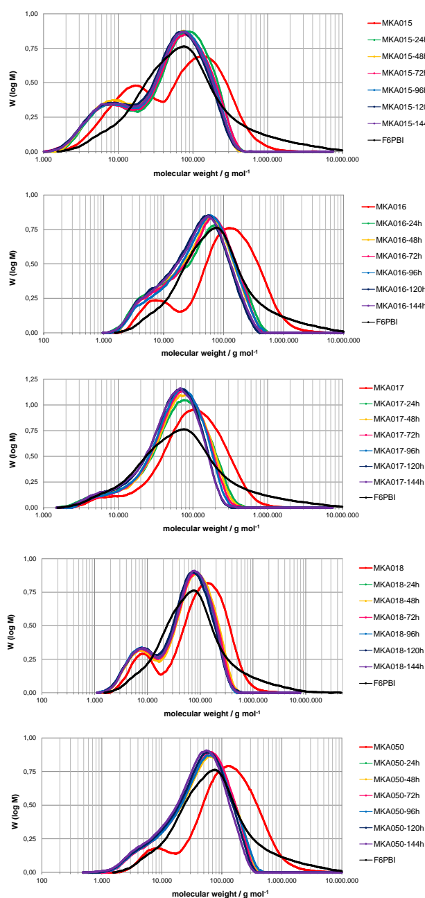
Fig. 7 M_w distribution of the MKA membranes before and after different durations of Fenton Test.
