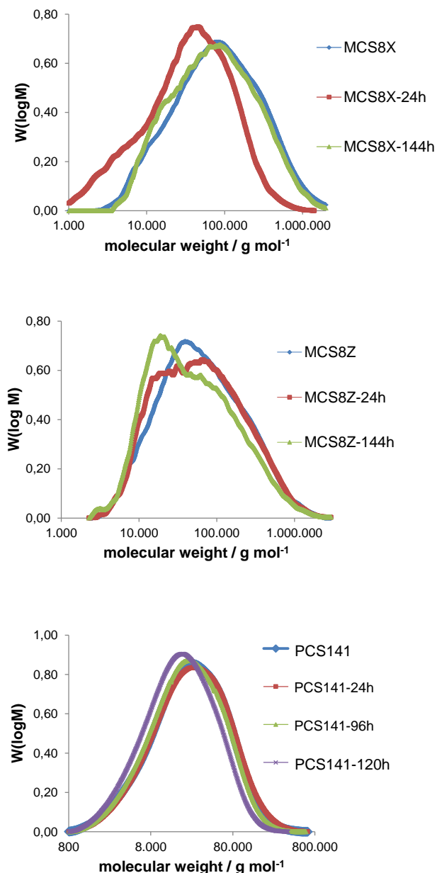
Fig. 6 M_w distribution of the membranes MCS8X, MCS8Z and PCS141 before and after different durations of Fenton Test.
