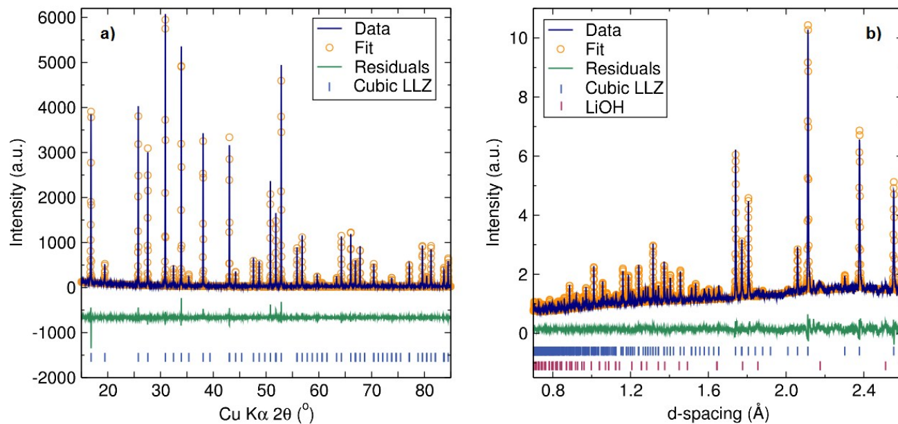
Fig. 1 Rietveld refinement to (a) PXR D and (b) backscattered detected NPD data collected on \text{Li}_{6.5}\text{Al}_{0.25}\text{La}_{2.92}\text{Zr}_2\text{O}_{12} . Fits were in excellent agreement to the cubic LLZ garnet in the (Ia\bar{3}d) space group. 24 (b) For the NPD data, a 2% LiOH impurity is also detected. 25
