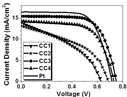
Figure 4. Characteristic J-V curves of DSSCs with cPTI-MCA-LiKCl-550 CEs and a Pt CE measured under simulated solar irradiation of AM 1.5 G ( 100 \text{ mW cm}^{-2} ).
