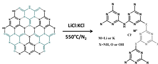
Scheme 1. Ionothermal synthesis of cPTI using MCA as a precursor.
