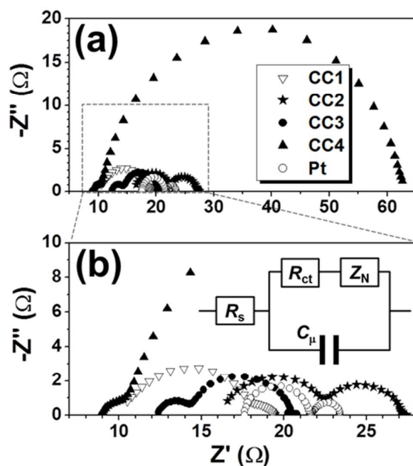
Figure 3. (a) Nyquist plot for the symmetrical cells, and (b) an expansion of the rectangle region of (a) and the equivalent circuit. The legend in (a) is for (b) as well.
