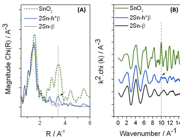
Figure 7 (A) magnitude of the Fourier transform spectra, and (B) EXAFS k^2 -weighted x data, of 2\text{Sn-}\beta , (black) and 2\text{Sn-h}^*\beta (blue). The corresponding spectra of \text{SnO}_2 (green dots) are also displayed.
