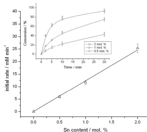
Figure 9 Catalytic activity of 2Sn- \beta for the MPV hydrogenation of cyclohexanone as a function of catalyst loading. Sn content was varied by changing the mass of 2Sn- \beta present in the reactor. Both the initial rate data (main figure) and the time online analysis as a function of Sn content within the reactor (inset) are presented.
