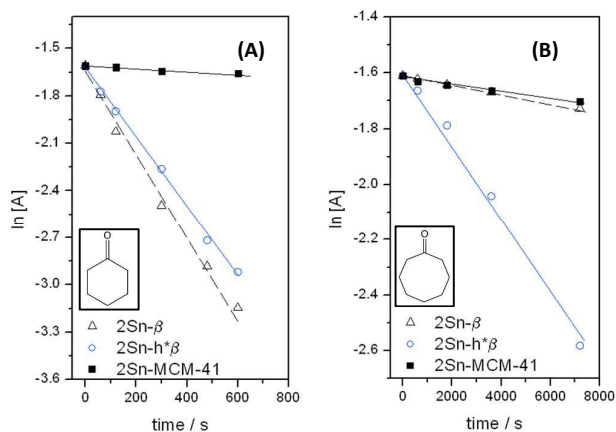
Figure 8 Catalytic activity for 2Sn- \beta (open triangles), 2Sn-h* \beta (open circles) and 2Sn-MCM-41 (filled squares) for the MPV reduction of (A) cyclohexanone and (B) cyclooctanone.
