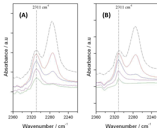
Figure 5 In situ DRIFTS spectra of (A) 2Sn-h* \beta , and (B) 2Sn- \beta , following (dashed) 10 minute treatment with CD 3 CN at room temperature. Various desorption temperatures (50 (red), 100 (blue), 150 (purple) and 200 °C (green)) are also displayed.
