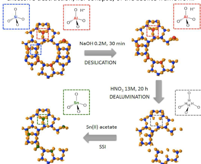
Figure 1 Postsynthetic desilication procedure for mesopores creation in the zeolite \beta using NaOH as desilication agent (step 1), and subsequent formation of stannosilicate via solid state stannation (step 2 and 3).
