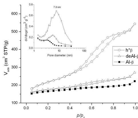
Figure 3 Porosimetry data for (black/squares) commercial Zeolite \beta , (hollow/triangles) deAl- \beta , and (hollow/circles) [deSi,deAl]- \beta (h* \beta ).
