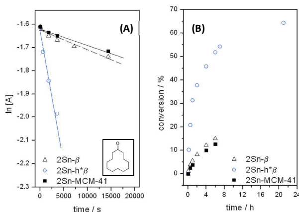
Figure 10 (A) Initial rate data for 2Sn- \beta (open triangles), 2Sn-h* \beta (open circles) and 2Sn-MCM-41 (filled squares) for the MPV reduction of cyclododecanone, and (B) extended time online profile for the same reactions.
