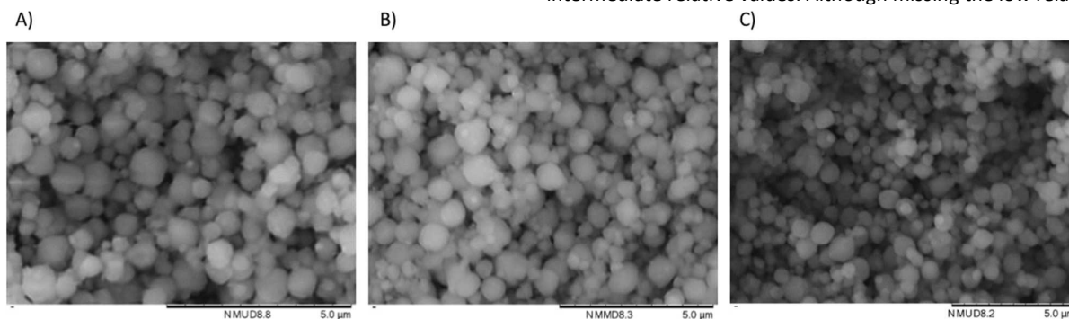
Figure 4 SEM images of A) commercial Zeolite \beta , B) 2Sn- \beta , and C) 2Sn-h* \beta .
