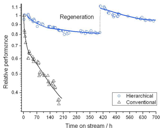
Figure 11 Catalytic activity for 2Sn- \beta and 2Sn-h* \beta for the MPV reduction of cyclohexanone in the continuous regime.
