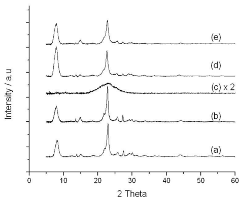
Figure 2 XRD patterns for (a) commercial Zeolite \beta , (b) deAl- \beta , (c) [deAl,deSi]- \beta , (d) [deSi,deAl]- \beta (h* \beta ) and (e) 2Sn-h* \beta .
