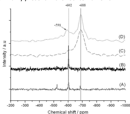
Figure 6 MAS NMR spectra of (A) \text{SnO}_2 , (B) 10 % \text{SnO}_2/\text{deAl-}\beta (physical mixture), (C) 2\text{Sn-}\beta , and (D) 2\text{Sn-h}^*\beta .
