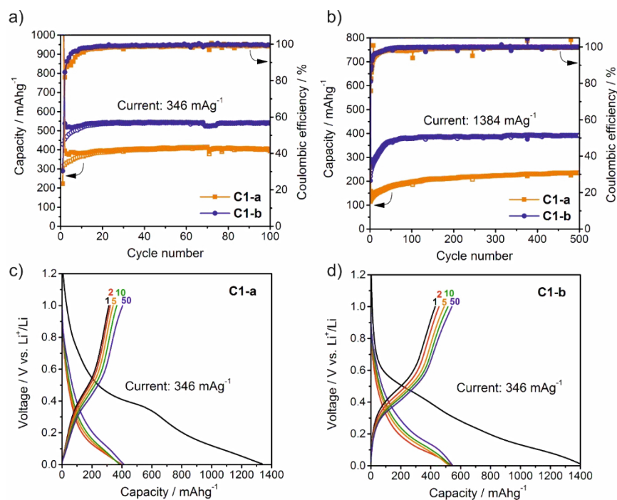
Figure 7 Electrochemical performance of Ge@C materials C1-a and C1-b as anode material for Li-ion batteries. The approximate size of germanium domains is (51±6) nm for C1-a and (13±1) nm for C1-b . a) Cycling stability at a current of 346 mA g -1 . b) Cycling stability at a current of 1384 mA g -1 . c) and d) Galvanostatic charge and discharge curves of composites C1-a and C1-b at a current of 346 mA g -1 . All cells were cycled in the potential range 0.005 – 1.0 V. Capacities and currents are related to the mass of the Ge@C composite corresponding to 80 % of the whole electrodes.
