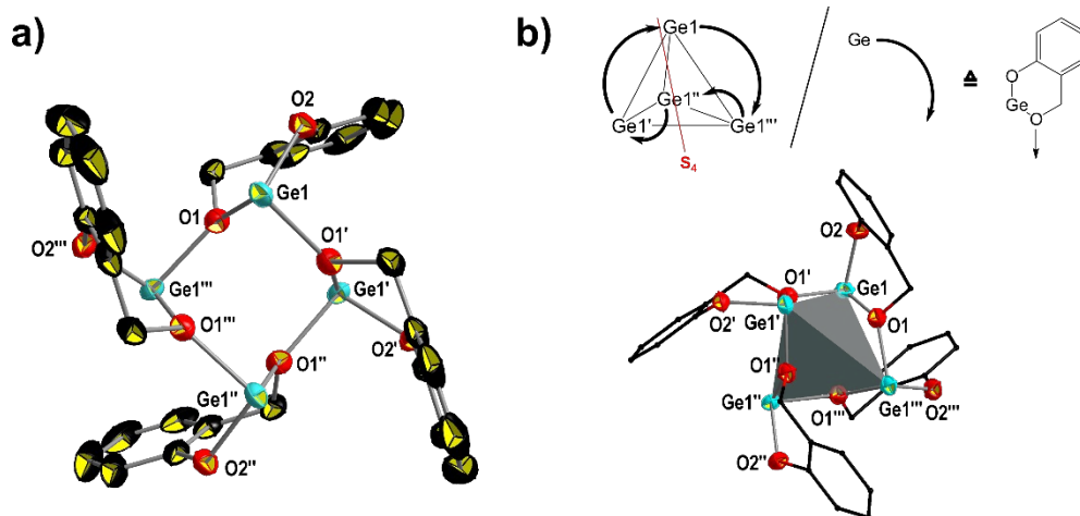
Figure 2 Molecular structure \alpha-(1)_4 a) in the solid state and b) with salicylic alcoholate moieties depicted in wireframe style and the tetrahedron spanned by the germanium atoms highlighted in grey. The scheme in b) illustrates the coordination pattern of the bridging benzylic oxygen atoms as indicated by the direction of the arrows. Thermal ellipsoids are drawn with 50% probability. Hydrogen atoms are omitted for clarity. Selected bond lengths [Å] and bond angles [°]: Ge1-O1 1.987(3), Ge1-O2 1.884(3) and Ge1-O1' 2.025(3); Ge1-O1-Ge1' 126.37(16), O1-Ge1-O2 91.36(13), O1-Ge1-O1' 85.29(14) and O2-Ge1-O1' 94.14(12). Symmetry transformations used to generate equivalent atoms: ' = x-0.5, -y+1.5, -z+0.5 ; '' = -x+2, -y+1, z ; ''' = -x+1.5, y+0.5, -z+0.5 .
