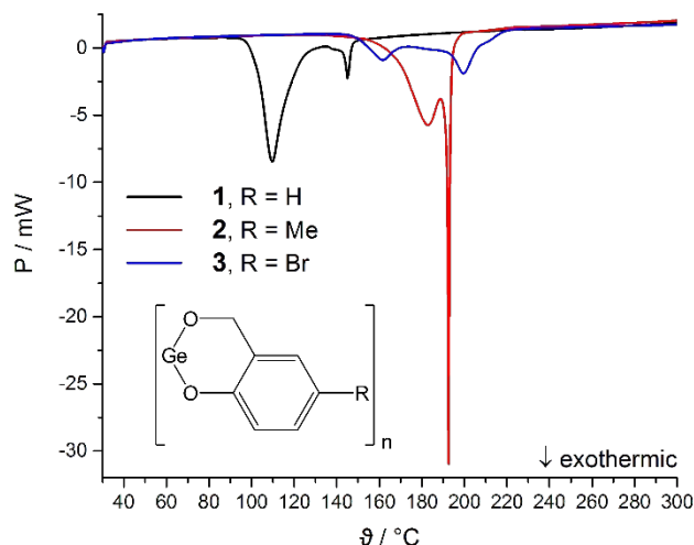
Figure 4 Differential scanning calorimetry of the amorphous materials of the germylenes 1 (black curve), 2 (red curve) and 3 (blue curve); heating rate 10 K min -1 , N 2 atmosphere, N 2 volume flow 50 mL min -1 .
