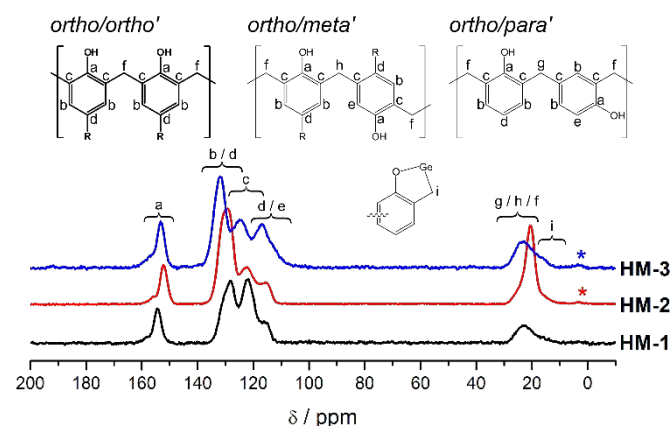
Figure 6 ^{13}\text{C}\{^1\text{H}\} CP-MAS NMR spectra of the germanium-containing phenolic resin hybrid materials as obtained by thermally induced twin polymerization of 1 - 3 . The spectra of HM-1 , HM-2 and HM-3 are depicted as black, red and blue lines, respectively. The asterisks * mark spinning side bands. Assignment of the resonance signals is given for the assigned connectivity patterns of the bridging methylene groups ( ortho/para' only for HM-1 ).
