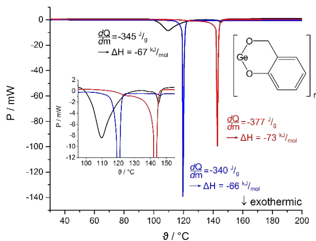
Figure 5 Differential scanning calorimetry of amorphous 1 (black curve), crystals of (1)_3 (red curve) and crystals of 2 \cdot (1)_4 \cdot n -pentane (blue curve); heating rate 10 K min -1 , N 2 atmosphere, N 2 volume flow 50 mL min -1 . The inset magnifies the range between 95 °C and 155 °C. The determined dQ/dm values and the as-calculated molar reaction enthalpies ( \Delta H ) that are referred to one monomeric unit of 1 of the exothermic processes are depicted in black for amorphous 1 , red for crystals of (1)_3 and blue for crystals of 2 \cdot (1)_4 \cdot n -pentane.
