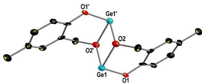
Figure 3 Molecular structure of (2)_2 in the solid state. Thermal ellipsoids are drawn with 50% probability. Hydrogen atoms are omitted for clarity. Selected bond lengths [Å] and bond angles [°]: Ge1-O1 1.862(7), Ge1-O2 1.986(6), Ge1-O2' 1.966(7); Ge1-O2-Ge1' 104.6(3), O1-Ge1-O2 91.6(3), O1-Ge1-O2' 94.9(3), O2-Ge1-O2' 75.4(3). Symmetry transformations used to generate equivalent atoms: ' = -x, -y+1, -z+1.
