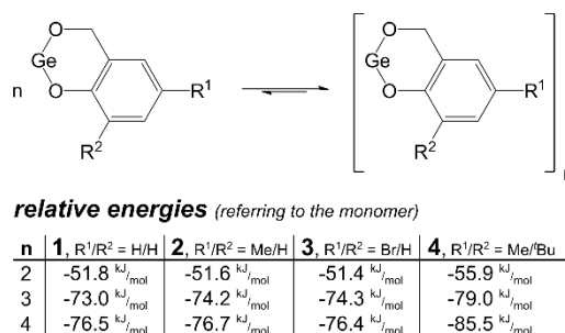
Scheme 2 Illustration of the equilibrium between oligomers of 1 - 4 in solution (top) and relative energies of the respective oligomers (bottom) calculated on the B3LYP-D3/def2-TZVPP level of theory with regard to the respective monomers.
