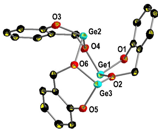
Figure 1 Molecular structure of (1)_3 in the solid state. Thermal ellipsoids are drawn with 50% probability. Hydrogen atoms are omitted for clarity. Selected bond lengths [Å] and bond angles [°]: Ge1-O1 1.8408(19), Ge1-O2 1.986(2), Ge1-O4 1.975(2), Ge2-O3 1.848(2), Ge2-O4 1.939(2), Ge2-O6 1.988(2), Ge3-O2 1.988(2), Ge3-O5 1.8447(19), Ge3-O6 1.951(2); Ge1-O4-Ge2 128.28(11), Ge2-O6-Ge3 115.94(10), Ge1-O2-Ge3 132.48(10), O1-Ge1-O2 92.45(9), O1-Ge1-O4 92.50(9), O2-Ge1-O4 86.80(9), O3-Ge2-O4 91.35(9), O3-Ge2-O6 97.57(9), O4-Ge2-O6 88.82(8), O2-Ge3-O5 97.60(8), O2-Ge3-O6 86.64(8), O5-Ge3-O6 92.77(9).
