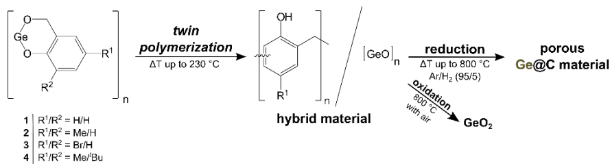
Scheme 1 Illustration of the basic structural motif of the germynes 1 - 4 ( n = 2 - 4 ) and the concept for the synthesis of e.g. a porous Ge@C material for rechargeable Li-ion batteries starting from 1 - 3 according to the concept of twin polymerization followed by reduction of the hybrid material.
