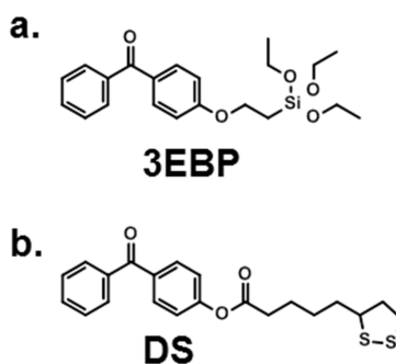
Figure 2. Surface cross-linkers used in this study. a) 3EBP forms self-assembled layers on any substrate that carries an OH group through Si-O bonds; [20] b) DS attaches to gold via S-Au bonds to form a monolayer. [21]
