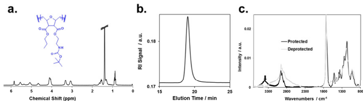
Figure 3. Characterization of the Propyl SMAMP precursor polymer and network: a) ^1\text{H} -NMR spectrum of the polymer, b) gel permeation chromatography elugram of the polymer; c) ATR-FTIR spectrum of the surface-attached precursor polymer network (protected) and activated polymer network (deprotected).
