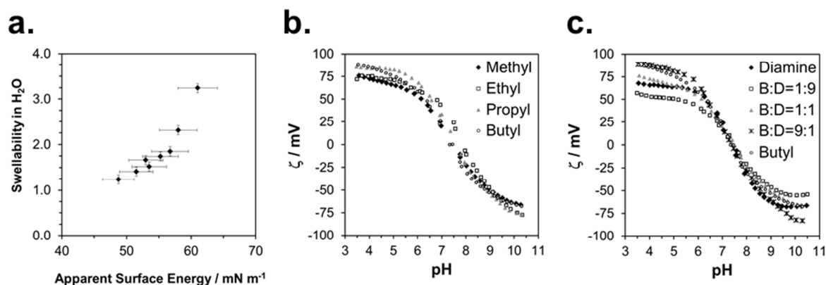
Figure 4. Physical characterization of the SMAMP networks: a) Correlation between swellability in water and apparent surface energy; b) Representative \zeta potential titration curves of the SMAMP homopolymer networks; c) Representative \zeta potential titration curves of the butyl SMAMP copolymer networks.
