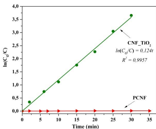
Fig.7 Kinetics of Rhodamine B degradation (linear transform \ln(C_0/C) vs. t ) in photocatalytic experiments using CNF_TiO 2 as photocatalyst in comparison with PCNF.
