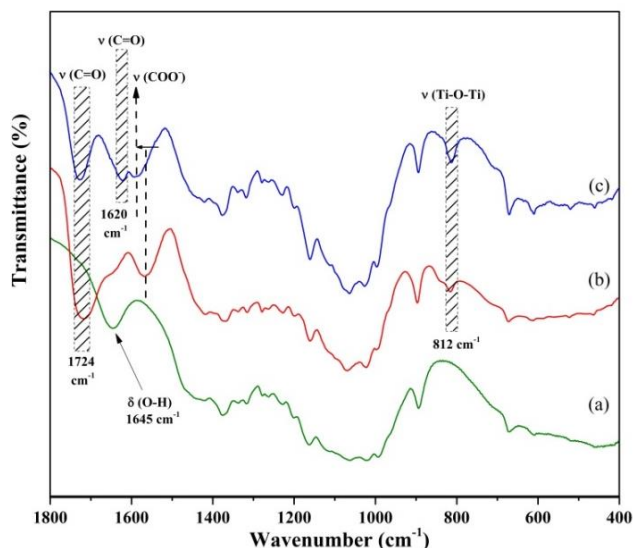
Fig.2 FTIR spectra of PCNF (a), CNF_ \text{TiO}_2 (b) and CNF_ \text{TiO}_2 _TC_M1 (c)
