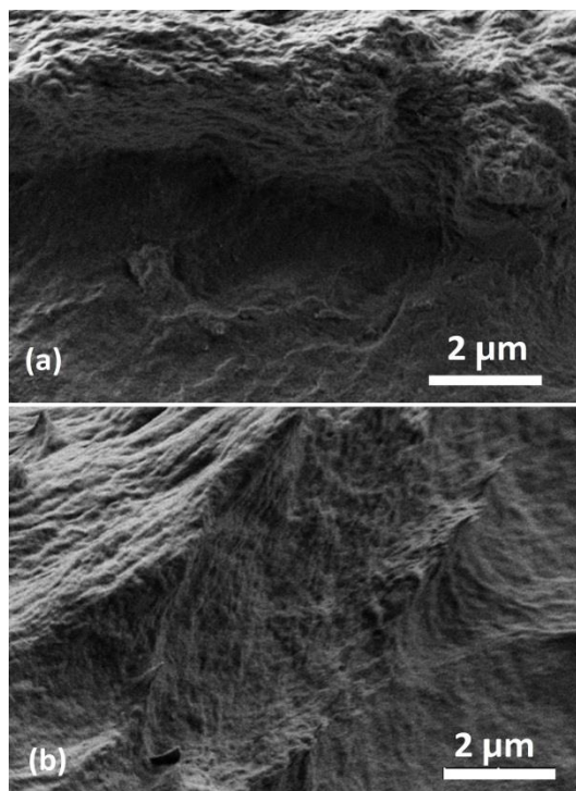
Fig.1 SEM images of the applied nanomaterials: (a) PCNF, (b) CNF_TiO 2
