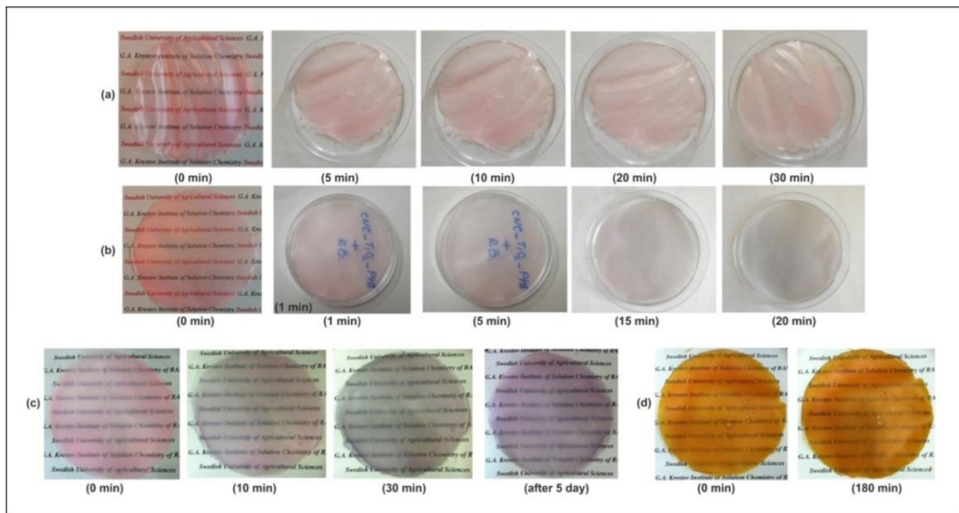
Fig.6 Photocatalytic activity of (a) PCNF, (b) CNF_TiO 2 , (c) CNF_TiO 2 _Phos_M2, (d) CNF_TiO 2 _TC_M1 under UV-irradiation
