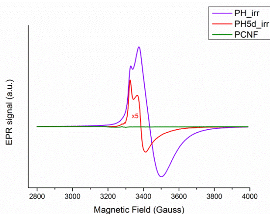
Fig.7 EPR spectra of PCNF (green), wet gel produced according to the CNF_TiO 2 _Phos_M2 method; PH_irr (blue), UV irradiated for 5 min using a 250 W lamp and PH5d_irr (red), same UV treatment as in PH_irr but stored for 5 days after irradiation (note that this spectrum is magnified for 5 times for easy comparison). EPR recording settings: Microwave frequency 9.29 GHz; power 20 \mu W. Modulation frequency 100 kHz; amplitude 10 G; T = 7 K.
