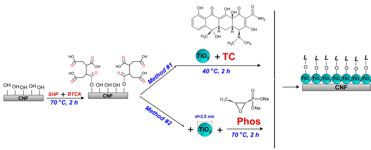
Scheme 1 Preparation of nanocomposites based on cellulose nanofibers and titania grafted with two types of drugs (TC and Phos – L) by two different methods: M1, M2 - method #1 and #2, respectively. SHP – sodium hypophosphite; BTCA - 1,2,3,4-butanetetracarboxylic acid
