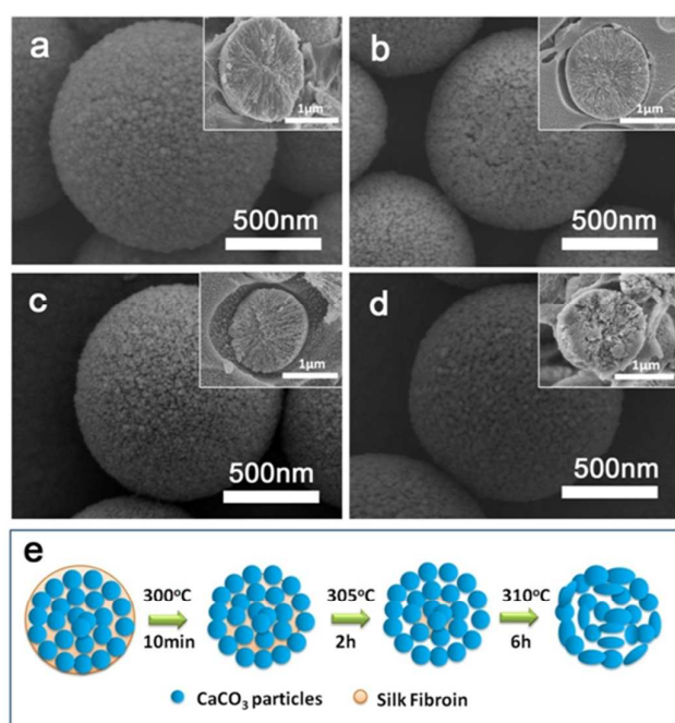
Figure 2. SEM images of silk-vaterite microspheres after different thermal treatments: (a) M-0; (b) M-300; (c) M-305; and (d) M-310; (e) Schematic diagram of the morphology changes for the silk-vaterite microspheres after different thermal treatments. The microspheres with size of 1-2 \mu\text{m} were composed of vaterite nanoparticles with diameter of tens of nanometers that could fuse following the removal of the silk. The inserts in (a-d) are cross-section images.
