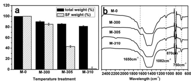
Figure 1. The weight and structural changes of the silk-vaterite microspheres after different thermal treatments: (a) The weight loss of the microspheres after thermal treatment when compared with the control (M-0). The original silk content inside the microspheres before thermal treatment was 10%, based on TGA curves of the particles from 0 to 800 °C at 10 °C min -1 in a nitrogen gas with flow rate of 40 cm 3 min -1 (The curves are not shown). (b) FTIR spectra of the CaCO 3 microspheres after different thermal treatments. The typical peaks of silk gradually decreased and almost disappeared following the increase of temperature and time while the peaks of vaterite keep stable in the processes.
