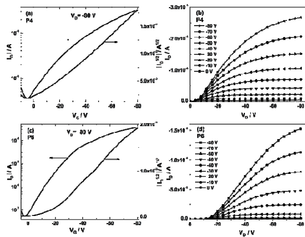
Figure 5. Transfer (a), (c) and output (b), (d) curves of P4 and P6 .
