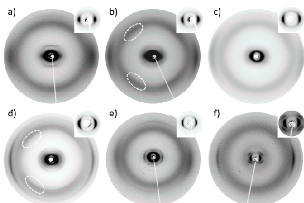
Figure 6. 2DWAXS patterns of a) P1 , b) P2 , c) P3 , d) P4 , e) P5 and f) P6 (insets show the small-angle scattering range). Off-meridional reflections related to a preferential organization of the alkyl chains are indicated in b) and d) by dashed circles.
