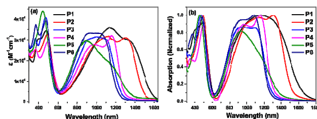
Figure 3. UV-vis-NIR absorption spectra of P1-P6 investigated in toluene solution (a) and in thin film (b).
