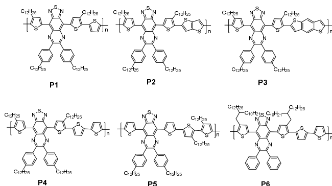
Figure 2. Structures of P1-P6 synthesized and studied in this work.
