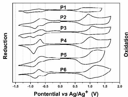
Figure 4. The reduction and oxidation curves of P1-P6 . The films were deposited from chlorobenzene solutions.
