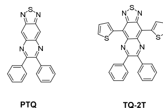
Figure 1. Structures of PTQ and TQ-2T reported in literature.
