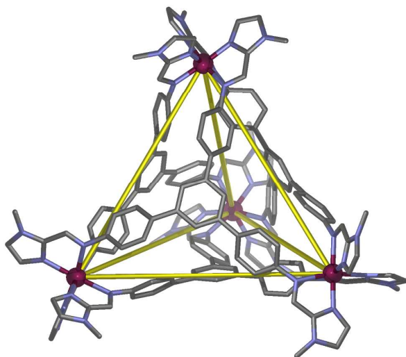
Figure 2 Schematic representation of the X-ray structure of cage 1 . Hydrogen atoms, anions and solvent molecules are not shown for clarity.
