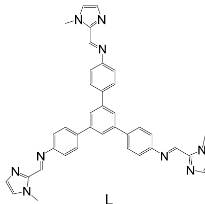
Figure 1 Schematic representation of rigid ligand L
