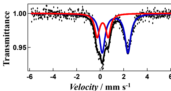
Figure 6: Mössbauer spectrum of non-solvated cage 1 at 5 K. The iron(II) high-spin is shown in blue, and low-spin in red.
