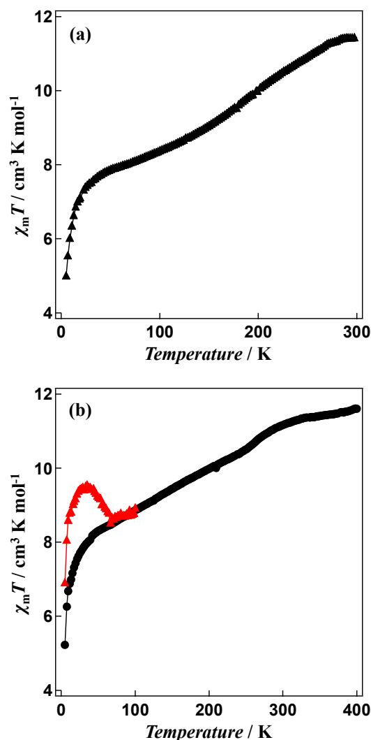
Figure 5 \chi_m T versus T plots for (a) solvated [\text{Fe}_4\text{L}_4](\text{BF}_4)_8 \cdot 16\text{CH}_3\text{CN} , the sample was measured in the temperature range between 5 K and 300 K and (b) non-solvated [\text{Fe}_4\text{L}_4](\text{BF}_4)_8 compound, the magnetic susceptibilities of the sample annealed at 400 K in the SQUID cavity was measured in the temperature range between 5 K
