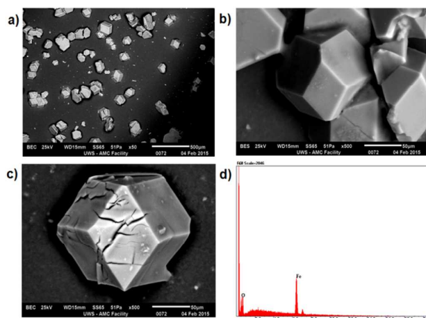
Figure 3. SEM images of crystals in polyhedral shape (a,b and c) and an EDS spectrum of cage 1 (d).
