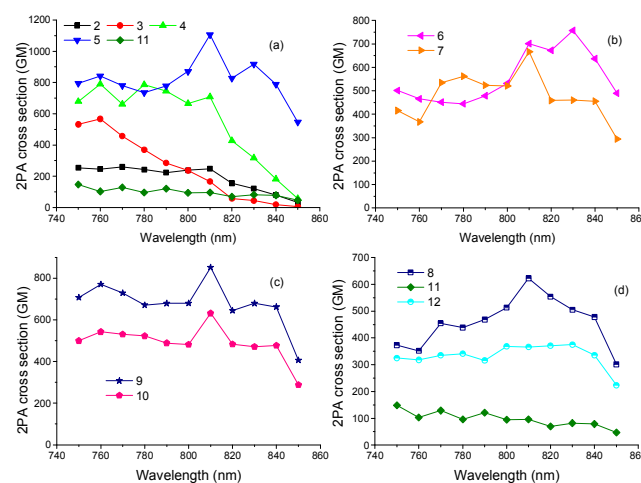
Fig. 5. Two-photon absorption cross-sections, \delta_{2PA} , of (a) 2, 3, 4, 5 and 11 (b) 6 and 7 (c) 9 and 10 and (d) 8, 11, 12 . All compounds have been measured in THF solutions at 10^{-4} M concentration.
