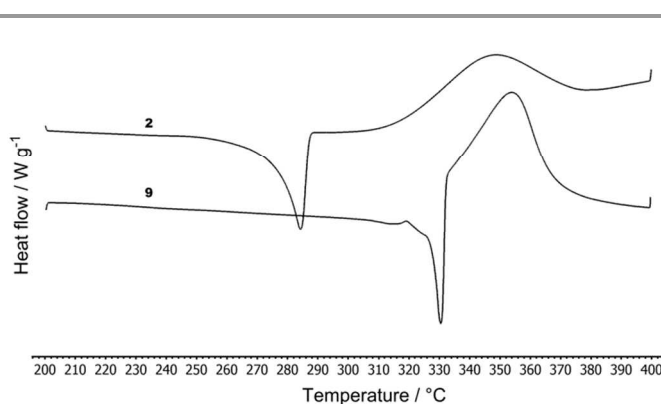
Fig. 3 Representative DSC curves of compounds 2 and 9 determined with a scanning rate of 3 °C/min under N 2
