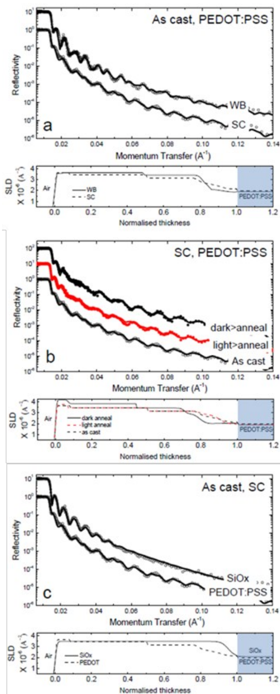
Figure 5. Neutron reflectivity data of PCDTBT:PC 60 BM system: (a) as cast SC and WBC films on PEDOT:PSS substrate; (b) SC films on PEDOT:PSS substrate in 'dark' and 'light' conditions after thermal annealing at 80°C for 1 hour; (c) as cast SC films on PEDOT:PSS and SiOx substrates
