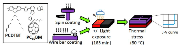
Figure 1. Schematic representation of processing PCDTBT:PC 60 BM blend with different coating techniques (SC and WBC) and light treatment. Chemical structures of PCDTBT and PC 60 BM are shown on the left box. Modest illumination ( < 10 \text{ mWcm}^{-2} ) is irradiated on film for a constant duration of 165 minutes prior electrode (Ca/Al) vacuum deposition. The devices and films without and with illumination are designated as "dark" (black colour) and "light" (red colour) conditions respectively in this study. The performance (J-V curve) of the fabricated devices is measured under 80^\circ C thermal stress.
