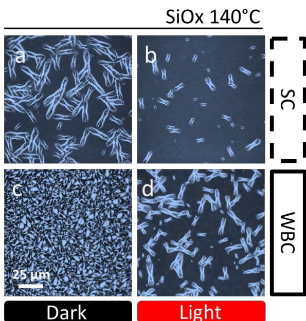
Figure 4. Optical microscope images of PCDTBT: PC 60 BM blend on PEDOT:PSS substrate annealed at 140°C for 1 hour. Films
