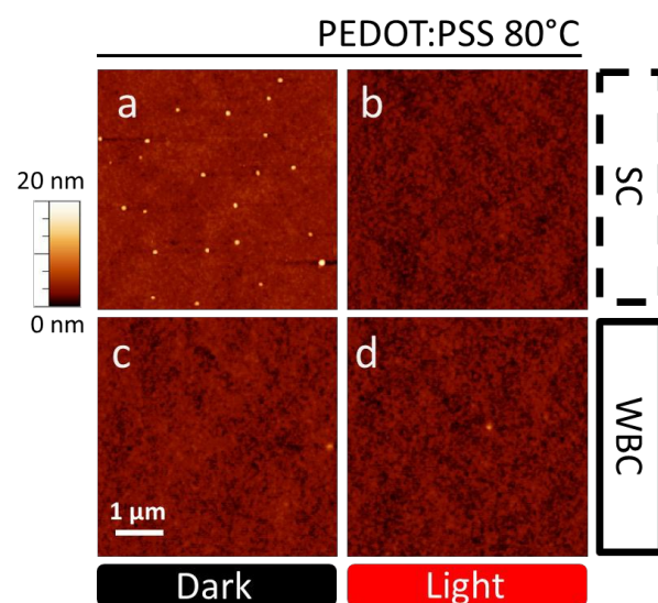
Figure 3. AFM images of PCDTBT:PC 60 BM blend on PEDOT:PSS substrate annealed at 80°C for 1 h. Films cast by (a), (b) SC and (c), (d) WBC and processed without (a), (c) and with (b), (d) prior light exposure.
