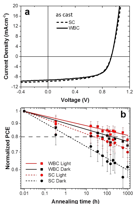
Figure 2. (a) Current density (J) – voltage (V) curves for typical PCDTBT:PC 60 BM blend devices processed with SC and WBC (prior to light processing) exhibiting PCE of 5.33 % and 5.26 % respectively (b) log:log plot of normalized PCE vs annealing time during thermal stress at 80^\circ C for devices fabricated via SC and WBC under dark and light processing conditions.
