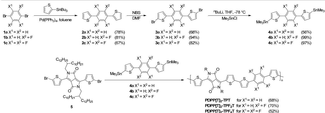
Figure 1: Syntheses of the thienophenylthiophene monomers with different degrees of fluorination. Experimental details are given in the Supporting Information. Synthesis of the extended PDPP-TPF n T copolymers by Stille-polycondensation. All yields are given in parentheses.
