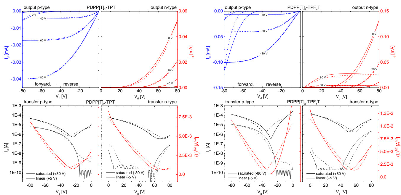
Figure 7. Representative OFET I - V curves in p-channel (blue output) and n-channel (red output) operation for the non-fluorinated PDPP[T] 2 -TPT (left) and the tetrafluorinated PDPP[T] 2 -TPF 4 T (right) after annealing at 350 °C. Solid lines represent forward scans, dashed lines the reverse scans in all graphs. In transfer curves (bottom), the black and gray plots indicate the transfer characteristics in the saturation and linear operation regime, respectively. I - V curves for the difluorinated PDPP[T] 2 -TPF 2 T as well as a scaled comparison of the n-output characteristics for all three polymers are given in the Supporting Information (Figure S9, Figure S10).
