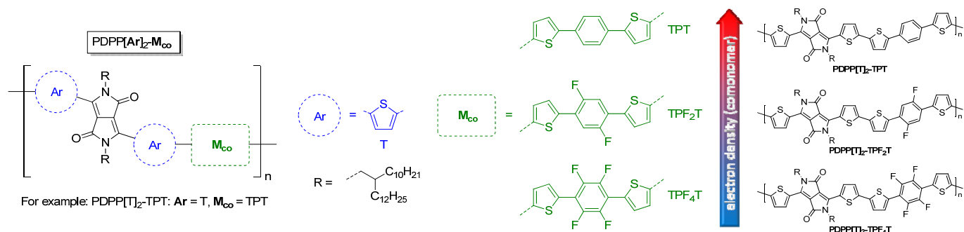
Figure 2: Structures of the new extended PDPP-TPF n T polymers in order of the overall electron density. R = 2-Decyltetradecyl (C 10 /C 14 ). The systematic nomenclature of the DPP copolymers is adopted from our earlier publication. 23
