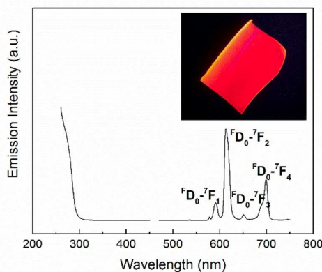
Fig. 5. Photoluminescence excitation ( \lambda_{em} = 615 nm) and emission ( \lambda_{ex} = 270 nm) spectra for a 100-nm thick Eu-hybrid thin film deposited at 290 °C on a quartz glass substrate; the inset shows a photo taken under 270-nm UV illumination of a similarly deposited film on an ITO-coated PET substrate.
