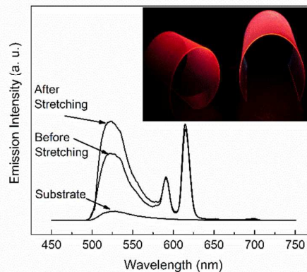
Fig. 7. Photoluminescence emission ( \lambda_{\text{ex}} = 270 \text{ nm} ) spectra for a 100-nm thick Eu-hybrid thin film deposited at 290 °C on a polyimide substrate before and after stretching; the inset shows a photo taken of this Eu-hybrid coating on a transparent polyimide substrate under 270-nm UV illumination.
