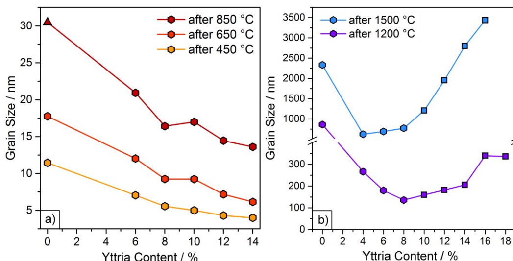
Figure 4. a) Grain sizes (obtained via XRD) as a function of Y content for particle samples Y6 to Y14 and undoped particle sample (Y0) 20 after heating at 450, 650 and 850 °C for 1 h. The monoclinic phase is represented by a triangle. All other samples were tetragonal or cubic. b) Grain sizes (obtained from SEM micrographs) of samples Y4 to Y18 and undoped sample (Y0) after heating at 1200 and 1500 °C for 3 h. The cubic phase is represented by squares. All other samples were tetragonal or monoclinic.
