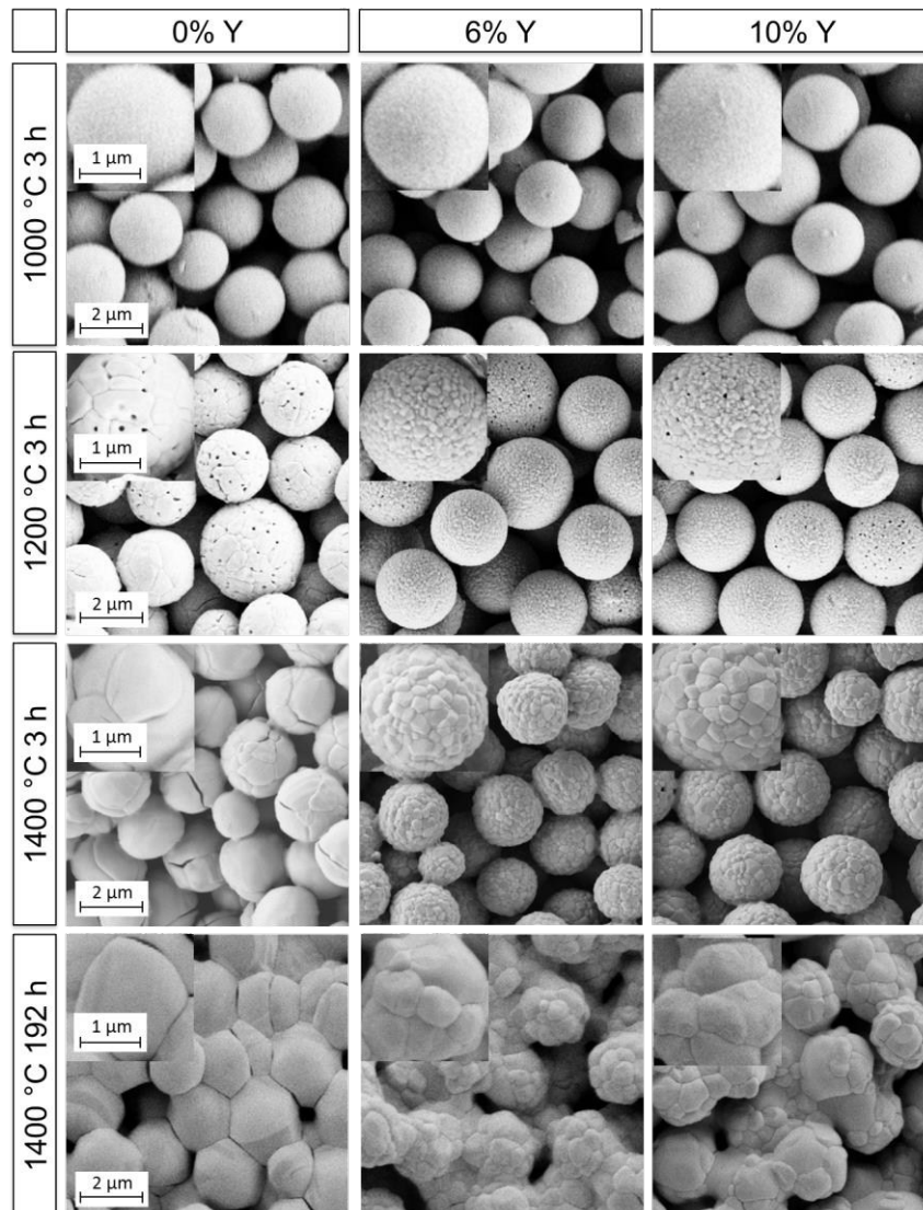
Figure 5. SEM micrographs of the films F0, F6 and F10 (left to right) after selected heating cycles. Scale bars apply to all images and insets within a given row.
