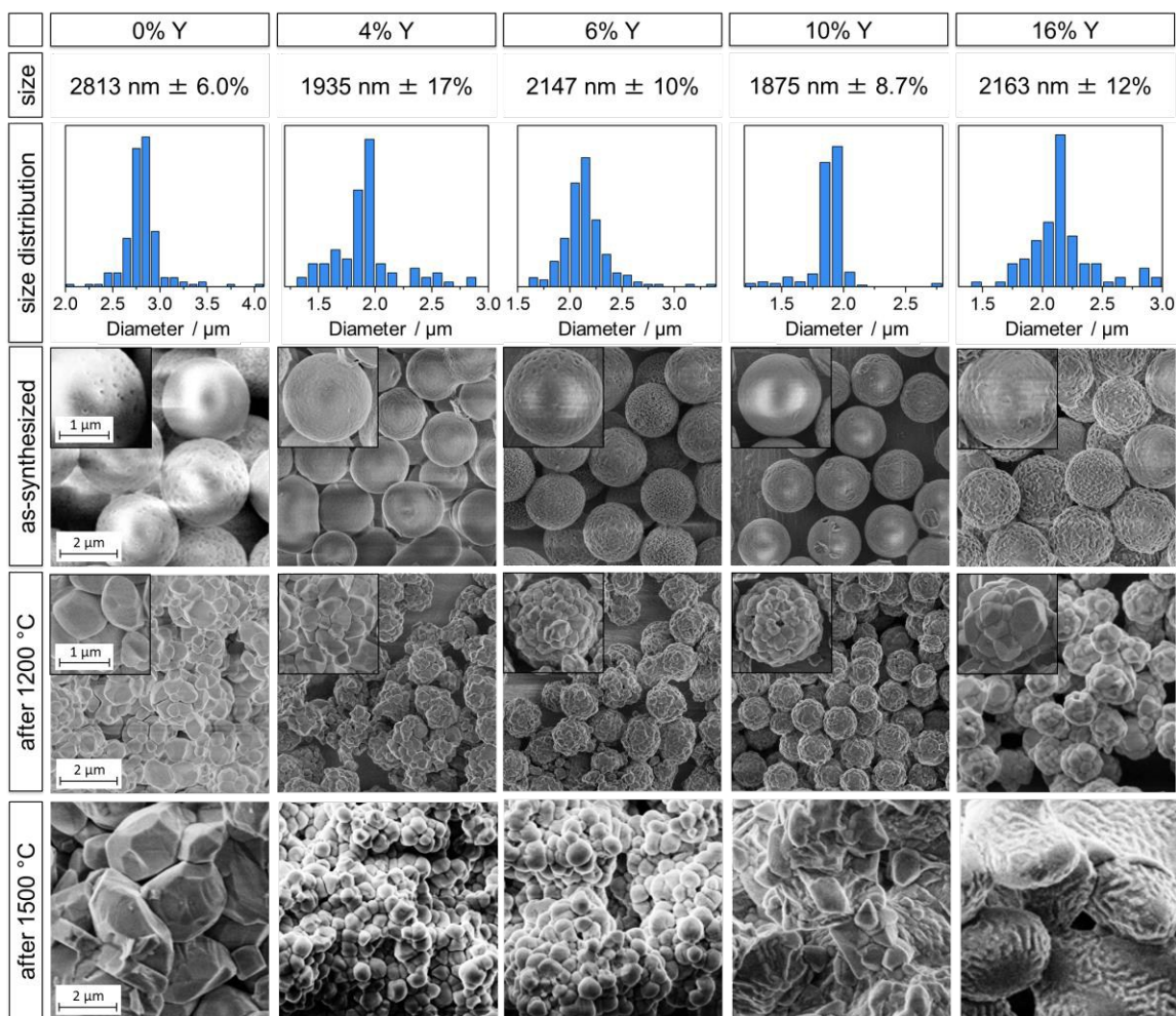
Figure 1. Undoped zirconia microparticle sample (0% Y) and yttria-stabilized zirconia particles with added yttrium amounts of 4, 6, 10, and 16% (from left to right). Diameter sizes with standard deviations (first row), size distributions (second row), SEM images of as-synthesized particles (third row), of particles heated at 1200 °C for 3 h (fourth row) and particles heated at 1500 °C for 3 h (fifth row). The undoped sample corresponds to B2.8 in prior work. 20 Scale bars apply to all images and insets within a given row.
