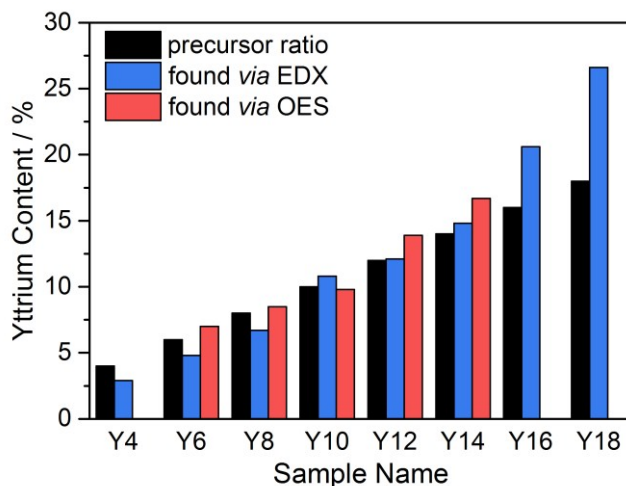
Figure 2: Target Y content (black) and Y contents measured via EDX (blue) and ICP-OES (red) for YSZ samples Y4 to Y18.
