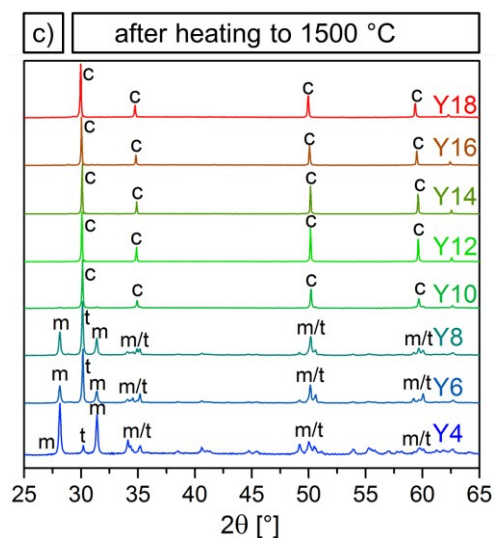
Figure 3. X-ray diffractograms of samples Y4–Y18 (bottom to top) after heating at 1200 °C for 3 h (a), an inset showing the transition from tetragonal to cubic for samples Y6–Y10 (b), and X-ray diffractograms for samples Y4–Y18 after heating at 1500 °C for 3 h (c). The tetragonal (t), monoclinic (m) and cubic (c) phases are indicated and labeled with their characteristic peaks.
