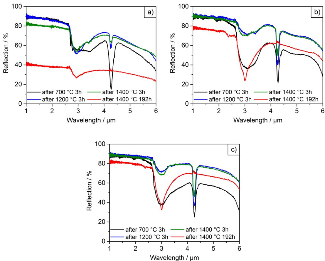
Figure 6. Diffuse reflectance spectra of films F0 (a), F6 (b) and F10 (c) after selected heating cycles.
