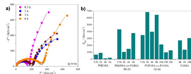
Figure 5. Behaviour of the R_{PB} as a function of thickness: a) complex plane plot for a representative brushes PHEMA-co-PAMA, b) comparison among the series. These data were obtained in presence of the redox probe (3 mM).
