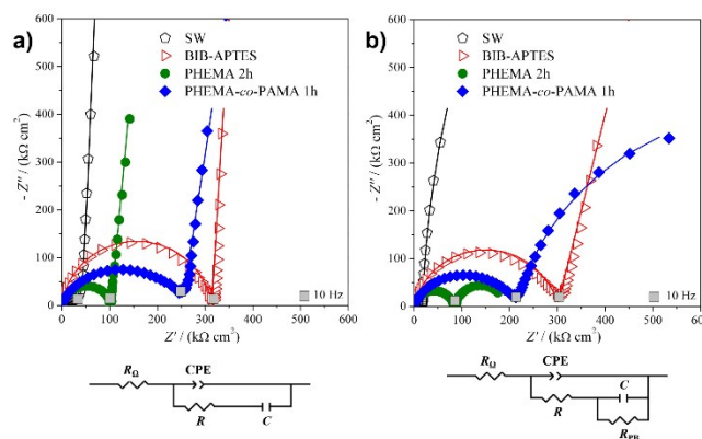
Figure 2. Complex plane plots measured for bare (SW) and initiator-functionalized (BIB-APTES) silicon wafer and for two representative brushes, along with the equivalent electrical circuits used for the interpretation of EIS plots, obtained a) in the absence and b) in the presence of redox probe.
