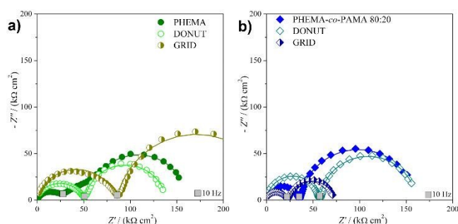
Figure 6. Complex plane plots showing the effect of patterning in the presence of redox probe (3 mM).
