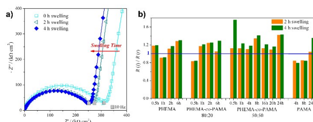
Figure 3. A) Complex plane plots showing the swelling of 1 \mu m-thick PHEMA- co -PAMA 80:20 brushes. b) Comparison of the swelling behaviour for all the investigated brushes.
