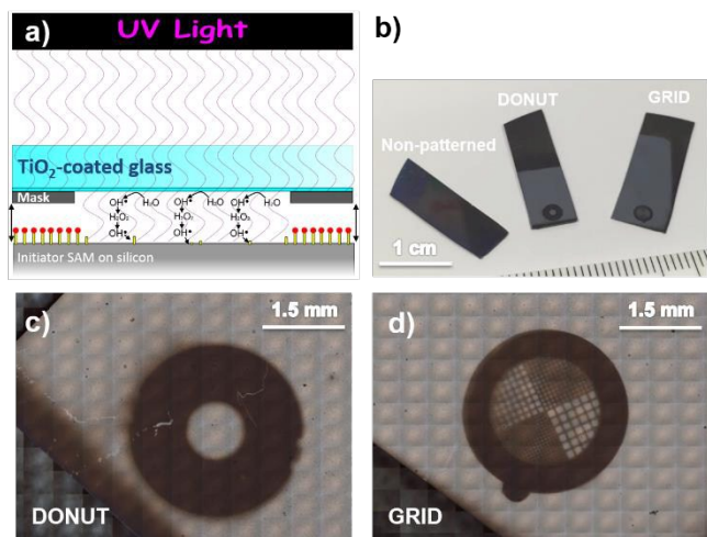
Figure 1. a) Scheme of remote photocatalytic lithography. b) Photographs of three representative samples, non-patterned and patterned. c) Optical microscopy images of donut-patterned (DONUT) and grid-patterned (GRID) brushes.
