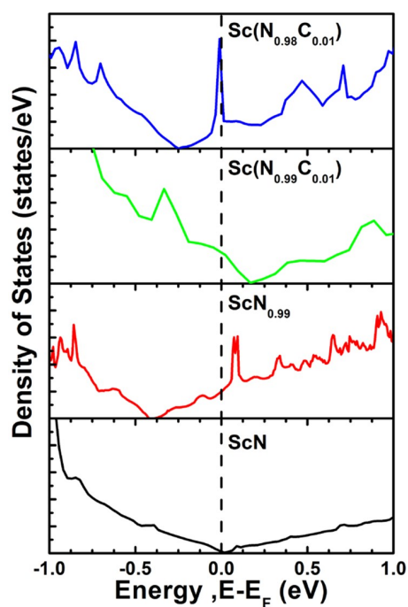
Figure 3. Example of effects of vacancies and dopants on the band structure of ScN (adapted from Ref. 46). Bottom: pure, stoichiometric ScN (note the inaccurate bandgap determination with GGA). Second from bottom: 1% N vacancies. Second from top: 1% C dopants. Top: Both C dopants and N vacancies.
