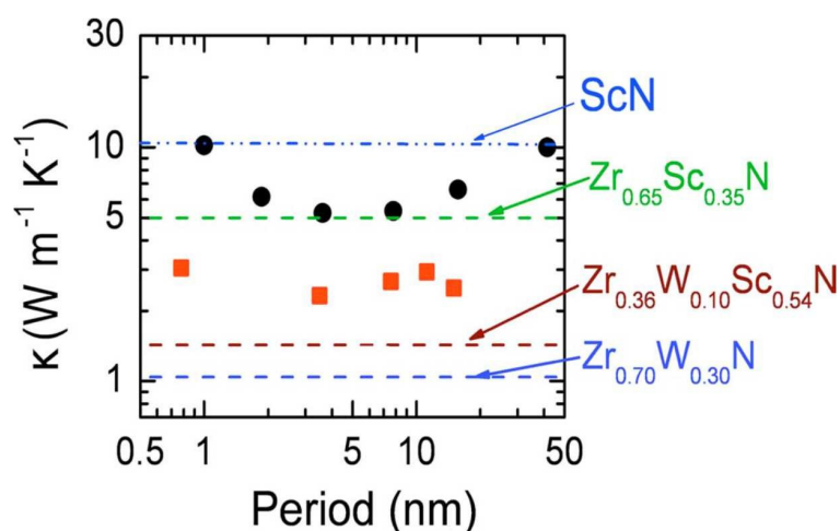
Figure 4. Illustration of superlattice reduction in thermal conductivity, from Rawat et al. 44 . Cross-plane thermal conductivity of 300 nm thick ZrN/ScN (dots) and Zr 0.64 W 0.36 N/ScN (squares) multilayers. Superimposed on the plot are horizontal lines corresponding to the experimentally determined lattice component of thermal conductivity, i.e., the alloy limit of different alloys of ZrN, ScN, and W 2 N. (Copyright American Institute of Physics, used with permission).
