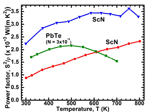
Figure 2. Thermoelectric power factor S^2\sigma of ScN (the bottom curve shows our first data from Ref. 2 and the top curve are the data of Burmistrova et al. 3 . The example data for PbTe are adapted from Sootsman et al. 43
