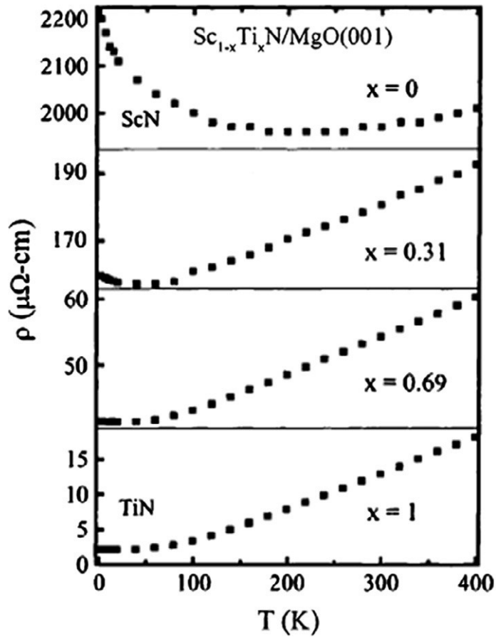
Figure 1. Electrical properties of ScN, TiN, and ScTiN alloys. From Gall et al. 22 (Copyright American Institute of Physics, used with permission).
