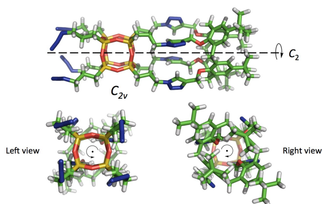
Figure 3. Minimum energy conformer of 5 optimized using the semiempirical PM3 method, showing the observed C_{2v} symmetry with the calixarene in a pinched-cone conformation.
