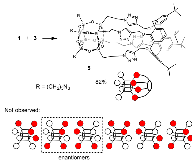
Scheme 2 Reaction conditions: 3 (0.2 equiv), [\text{Cu}(\text{C}_{18}\text{tren})]\text{Br} , i\text{Pr}_2\text{NEt} , toluene, 50 °C, 20 h.
