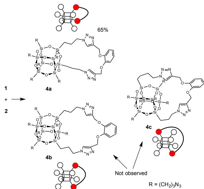
Scheme 1 Reaction conditions: 2 (0.2 equiv), [\text{Cu}(\text{C}_{18}\text{tren})]\text{Br} , i\text{Pr}_2\text{NEt} , toluene, 50 °C, 20 h.
