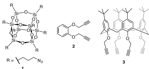
Figure 1 Structures of the octa-azido silsesquioxane and polyalkynes used in this work.
