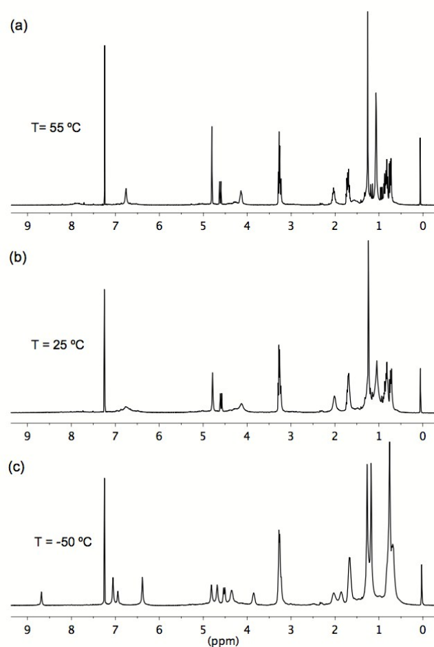
Figure 2. ^1\text{H} NMR spectra (400 MHz) of 5 in \text{CDCl}_3 at different temperatures.
