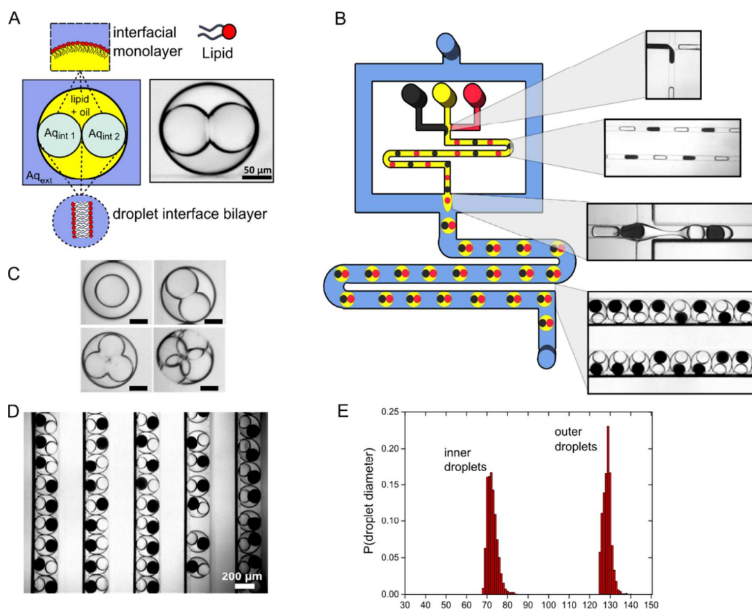
Fig. 1 – Microfluidic generation of multisomes. (A) Schematic of a multisome with bilayers present at all water-oil interfaces and corresponding brightfield images of different regions. First, alternating droplets of two different compositions are generated by two opposing T-junctions. These travel through a meander, allowing time for monolayer stabilisation. Two such droplets are then encapsulated downstream in an oil droplet using a flow-focussing channel geometry, generating two-droplet multisomes (C) By altering the generation frequencies of the internal aqueous droplets, 1,2,3, and 4 compartment multisomes can be generated (D) Monodisperse two-droplet multisomes with different inner droplet compositions stored in collection channels. Black droplets contain methyl-blue dye. (E) Inner and outer droplet size distribution for two-droplet double emulsion.
