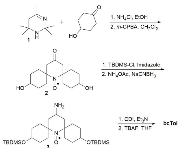
Scheme 1 Synthesis of bcTol . TBDMS-Cl tert-butyltrimethylsilyl chloride; CDI, carbonyldiimidazole.
