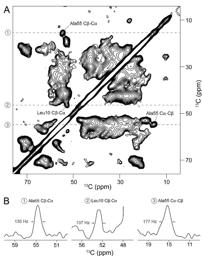
Fig. 3 DNP enhanced ^{13}C - ^{13}C correlation spectrum of microcrystalline SH3 at 100 MHz carbon frequency (at 9.4 T), recorded at 181 K. (A) 2D ^{13}C - ^{13}C DARR spectrum recorded with 25 ms mixing time. The dashed lines indicate positions of cross sections for evaluation of line widths. (B) Cross sections for selected cross peaks as indicated in (A), along with their line widths. To enable the evaluation of line width, the spectrum was recorded with a sufficiently long acquisition time and processed without application of a window function in F_2 .
