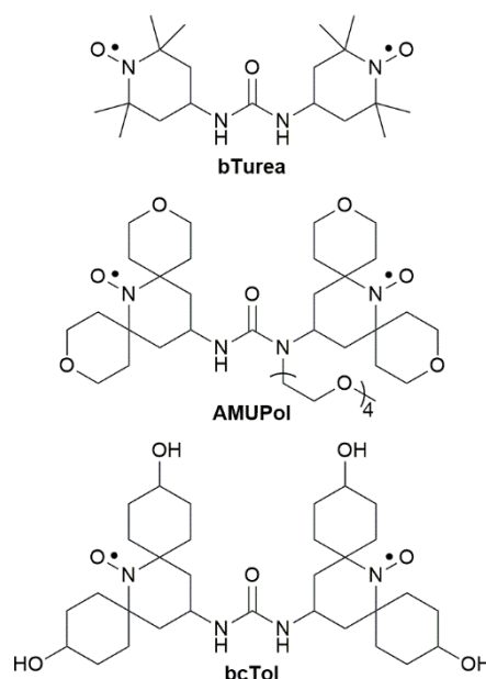
Fig. 1 Structures of bTurea, AMUPol and bcTol.
