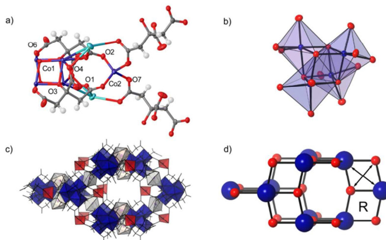
Figure 1 a) Citrate-encapsulated cubane units are linked by Co tetrahedra; b) Co1 atoms are linked by oxygen atoms O1, O3, O4, and O6 to form S_4 -symmetric \text{Co}_4\text{O}_4 cubanes; c) Polyhedral representation of UTSA-16, \text{Co}_4\text{O}_4 units are shown in blue, Co tetrahedra in red, and irregular K polyhedra in white; d) Structure of anatase, I4_1/amd , (Ti - Blue, O - Red) whose topology is analogous to UTSA-16. 'Wine-rack' rings indicated with 'R', diagonals indicated with arrows.
