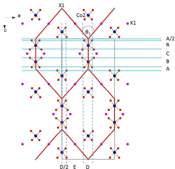
Figure 4: Simplified view of the structure showing only the tetrahedra based on Co2, the centroids of the Co1-based cubanes and the potassium ions. Division of the c -axis into regions A, B and C, and division of the a -axis into regions D and E is also shown. The diamondoid lattice referred to in the text is shown in red.
