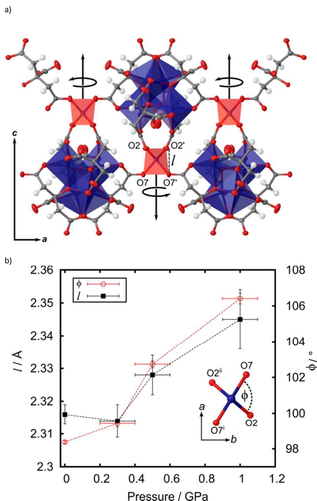
Figure 3 a) NLC arises along the c axis by the elongation of the Co tetrahedra, a result of the twisting of the O-Co-O planes. In order to maintain Co-O bond lengths, the tetrahedron height, l , must increase; b) Increase in dihedral angle \phi and consequential increase in tetrahedron height l with increasing pressure.
