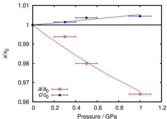
Figure 2 Normalised changes in unit cell dimensions with pressure. 2nd-order Birch-Murnaghan equations of state are represented as dashed lines. The error bars in the vertical axis are smaller than circles used for the data points.
