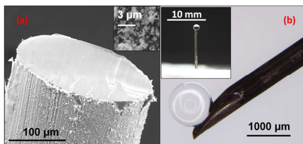
Fig. 1: Image (a) is a SEM image at 1000 \times magnification showing a SHP copper wire support (with SHP coated sides and a bare copper tip). The inset shows the rough surface of the SHP coating at 36600 \times . Image (b) shows a SHP coated GC syringe needle with a 0.5 \mu\text{L} droplet sitting as a "ball" at the tip. The inset shows a SHP support holding a 0.5 \mu\text{L} water droplet.
