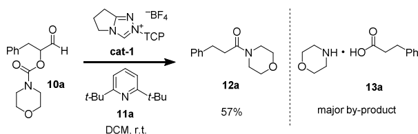
Scheme 6: Intramolecular variant of direct redox amidation.
