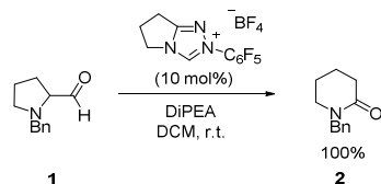
Scheme 2: Gravel's NHC catalyzed redox lactamisation. 27
