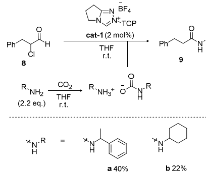
Scheme 5. Examples of direct NHC-catalysed amidation using substrate 8 .
