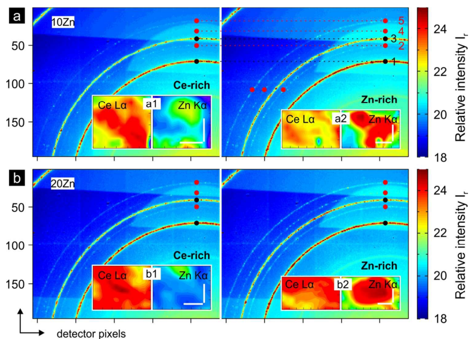
Fig. 5 Synchrotron 2D \mu -XRD patterns of (a) 10Zn and (b) 20Zn after 4 \text{H}_2\text{O} -splitting cycles. Left column: patterns for Ce-rich regions (a1, b1). Right column: patterns for Zn-rich regions (a2, b2). The insets show corresponding cerium and zinc XRF maps of the regions, with scale bars all representing a length of 20 \mu\text{m} . Black dots “1” and “3” represent \text{CeO}_2 (111) and (200). Red dots “2”, “4” and “5” represent ZnO (100), (002) and (101), respectively. The relative diffraction intensity ( I_r ) shown in the figure is the logarithm (base 2) of the intensity counts.
