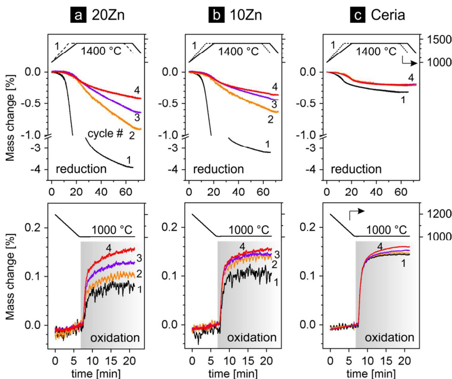
Fig. 9 TGA profiles of 4 thermochemical CO 2 -splitting cycles with (a) 20Zn, (b) 10Zn and (c) native ceria. Top row: mass loss profiles during reduction at 1400 °C, and bottom row: mass gain profiles during reoxidation (grey region) at 1000 °C by CO 2 .
