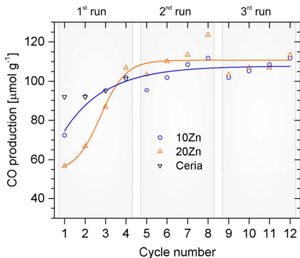
Fig. 10 CO production per gram of materials during 12 CO 2 -splitting cycles (three consecutive runs with 4 cycles per run) with reoxidation at 1000 °C and thermal reduction at 1400 °C.
