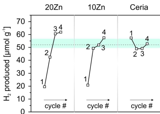
Fig. 3 Comparison of H_2 productivity at 1000 °C by native ceria, 10Zn, and 20Zn during 4 H_2O -splitting cycles. The colored band indicates the range of native ceria's productivities and the dashed line indicates the average value.
