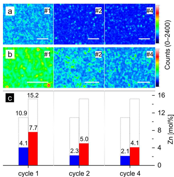
Fig. 4 Zinc XRF maps of (a) 10Zn and (b) 20Zn after 1, 2 and 4 H 2 O-splitting cycles. The scale in each map represents a length of 500 \mu\text{m} . Corresponding average zinc concentrations (blue: 10Zn, red: 20Zn) are presented in (c). The concentrations of zinc in the starting materials (bars with dashed lines) are included for comparison.
