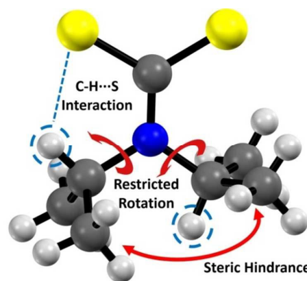
Figure 1. Structure of the dipdtc anion showing the important interactions.
