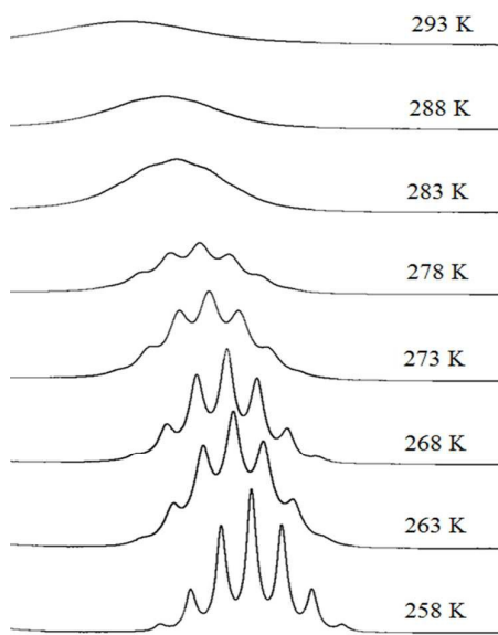
Figure 7: Selected portion of the 600 MHz ^1\text{H} spectra for \text{Na}(\text{dipdctc})\cdot 5\text{H}_2\text{O} in \text{CD}_3\text{CN} , showing the change in H2 resonance as a function of temperature.
