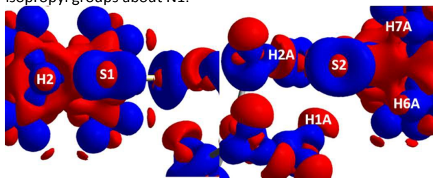
Figure 6: 3D Static deformation densities of the sulfur tori (viewed down the C-S bond).
