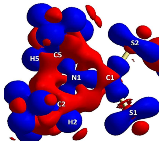
Figure 5: Theoretical 3D electrostatic densities of the Na(dipdte)·5H 2 O anion at the B3LYP 6-311G( d,p ) level. Areas of lower density are shown in red, and areas of higher density are shown in blue.
