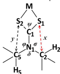
Figure 8. Depiction of the important distances and angles discussed in the text.
