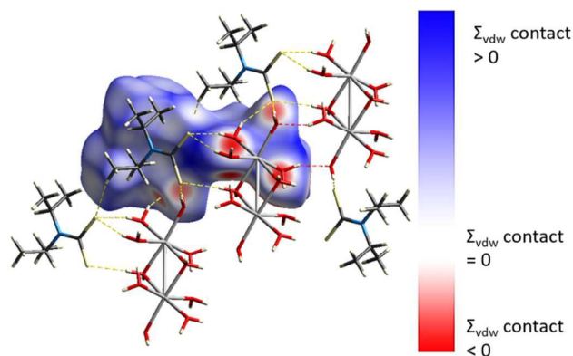
Figure 4: Hirshfeld surface and O-H...S hydrogen bonds (yellow) and O-H...O hydrogen bonds (red).
