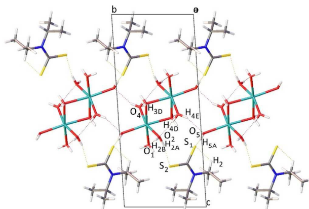
Figure 3: Molecular packing diagram as viewed along the a axis, showing layered morphology of Na(dipdctc)·5H 2 O.
