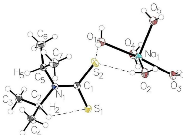
Figure 2: The structure of the Na(dipdctc)·5H 2 O asymmetric unit showing the atom-labelling scheme and thermal displacement ellipsoids at 50% probability.
