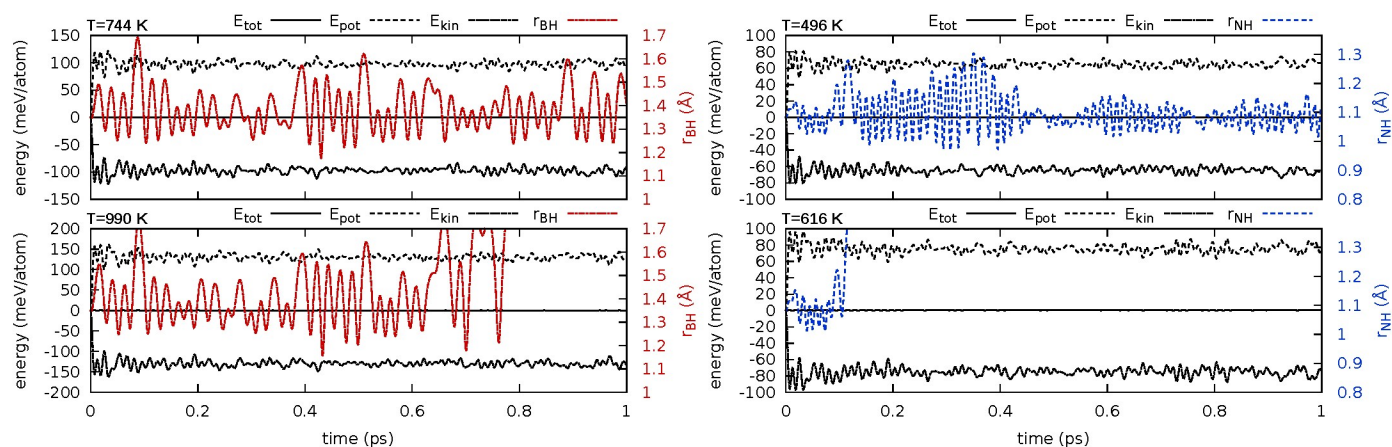
Fig. 5 NVE molecular dynamics of 1\alpha (left) and 1\beta (right). Black solid, dashed and dash-dotted line represent total, potential and kinetic energy (with E(t=0) = 0 ). The given T is the time-average over the last 0.5 ps. Initial kinetic energies are 1500 and 2000 K for 1\alpha and 1000 and 1200 K for 1\beta
