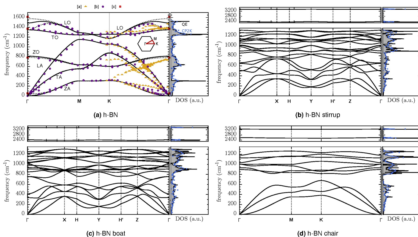
Fig. 7 DFT-PBE phonon dispersion of (a) pristine h-BN, and hydrogenated h-BN in the (b) stirrup, (c) boat and (d) chair configuration. The reciprocal space paths are explained in Fig. 8. [a]=Rokuta et al. 43 (HREELS), [b]=Serrano et al. 44 (inelastic x-ray scattering) [c]=Geick et al. 45 , Nemanich et al. 46 , Reich et al. 47 (Raman and IR at \Gamma ). Solid (dashed) lines are for monolayer (bulk). The DOS shown is that of monolayer h-BN. Blue lines and squares give the DOS from supercell calculations (CP2K) as Gaussian broadening (width 25 \text{cm}^{-1} ) or histogram (25 \text{cm}^{-1} intervals) respectively
