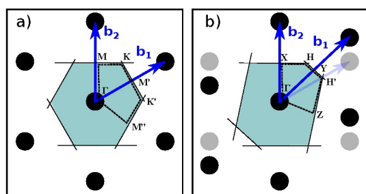
Fig. 8 Construction of the Brillouin Zone and high symmetry points. Pristine h-BN and \Gamma_2 have a hexagonal unit cell (a), with (in 2D) \mathbf{b}_1 = (1, 1/\sqrt{3}) and \mathbf{b}_2 = (0, 2/\sqrt{3}) in units of 2\pi/a . \Gamma_2 and \Gamma_3 have a monoclinic cell (b) with \mathbf{b}_1 = (1, -1/\tan \gamma) and \mathbf{b}_2 = (0, a/b \sin \gamma) . The constructed path in terms of reciprocal unit vectors ( \mathbf{b}_i ) is given by \Gamma = (0, 0) , X = (0, 1/2) , K = H = (1/3, 1/3) , Y = (1/2, 0) , H' = (2/3, 1/3) and Z = (1/2, -1/2) . M and K refer to the hexagonal cell ( \gamma = 120^\circ , a = b )
