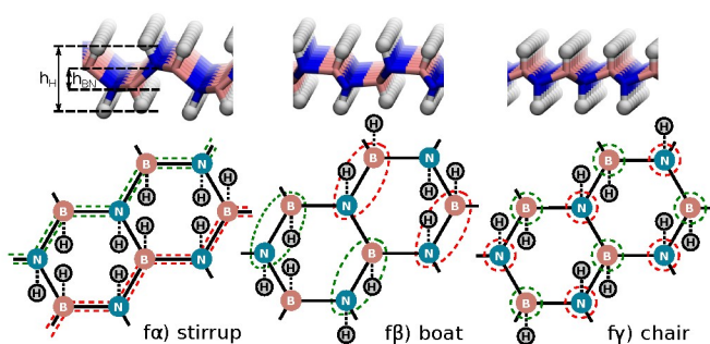
Fig. 2 Side view and schematic illustration of fully hydrogenated h-BN configurations. Red (green) dashed lines indicate B or N atoms with H atoms above (below) the h-BN sheet
