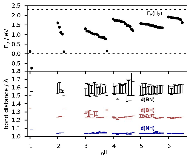
Fig. 4 E_b and bond distance range as a function of the number of H atoms in a hexagon ( n^H ). d(\text{BN}) is the distance from B/N atoms bound to H to any neighbouring B or N atoms. For visualization purposes, points for a given n^H are spread over a larger interval
