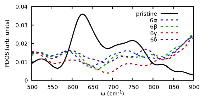
Fig. 10 Vibrational DOS in the range 500 – 900 \text{cm}^{-1} . The DOS is projected onto B and N atoms in the hexagon where H is chemisorbed
