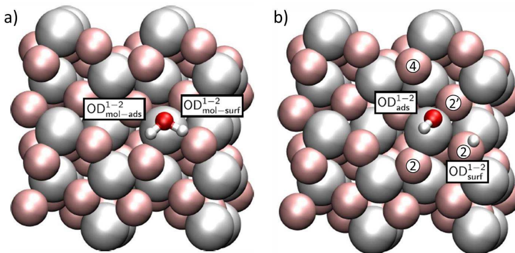
Fig. 4 Adsorption geometries for a) molecular and b) dissociated water in the 1-2 configuration. For convenience, surface atoms are shown as “van-der-Waals spheres” in pale colours, adsorbate species in a ball-and-stick representation. Possible adsorption sites are also designated in b).
