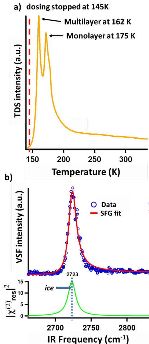
Fig. 2 a) the TPD spectrum of mass 20 ( D_2O ) for a sample, prepared as described in the text. To perform the TPD, after stopping D_2O dosing at 145 K we applied a heating ramp of 100 K/min and detected the desorption of mass 20. The desorption maximum at 162 K is assigned to water desorbing from the the weakly bond multilayer of ice (it can be increased in intensity by dosing for longer at low surface temperature). The peak at 175 K is assigned to monolayer desorption. Its amplitude is independent of low temperature dosing time. b) VSF spectrum of \alpha-Al_2O_3(1\bar{1}02) surface covered by D_2O ice and showing the characteristic free-OD peak of the ice/vacuum interface 12 .
