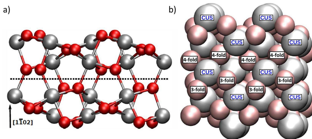
Fig. 1 (2 \times 2) supercell model of the oxygen terminated \alpha\text{-Al}_2\text{O}_3(1\bar{1}02) surface used in this study; oxygen atoms are shown as smaller red, aluminum atoms as larger grey balls. a) Side view (ball-and-stick representation): For further optimizations and vibrational analyses featuring adsorbate species on the top side of the slab atoms below the dotted line were kept fixed at their position initially optimized for the bare surface. b) Top view (“van-der-Waals spheres”): Aluminum positions for water adsorption are indicated with “CUS” labels. 1 rows of 3-fold and one of 4-fold coordinated oxygens are labelled for reference.
