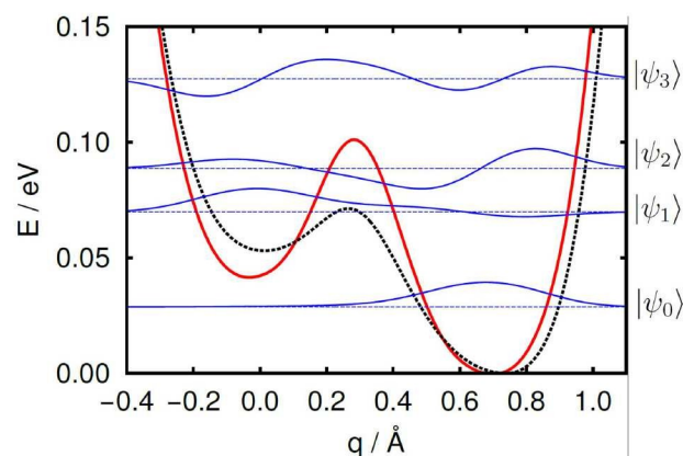
Fig. 9 NEB-derived potential for 1-4 water dissociation on the \alpha -Al 2 O 3 (1102) surface based on pure PBE (dotted black) and HSE06 (solid red). The latter was obtained by single-point calculations on PBE geometries; both potentials were aligned with respect to the 1-4 dissociated minimum ( i.e. the minimum on the right). Vibrational eigenvalues (dashed blue) and wave functions (solid blue) are given for the HSE06 potential; the reaction coordinate q is a projection onto the linear transit path between both minima (see text for details).
