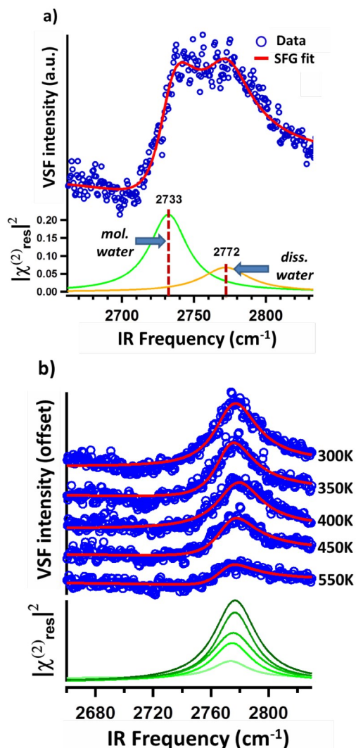
Fig. 3 VSF spectra of interfacial water at different surface temperatures. a) OD stretch spectra of a sample rapidly annealed to 185 K and immediately cooled to 135 K for characterization. The coverage is in the submonolayer regime. The spectrum clearly shows two features the lower frequency of which is assigned to molecularly, the higher frequency of which to dissociatively, adsorbed D_2O (see text for discussion). b) Series of VSF spectra collected from a \alpha\text{-Al}_2\text{O}_3(1\bar{1}02) rapidly annealed to the indicated temperature. Between each annealing step the sample is cooled to 135 K for VSF spectra characterization. Clearly only a single feature is apparent whose intensity decreases with annealing temperature. This feature is assigned to (an) OD stretch mode of dissociatively adsorbed D_2O
