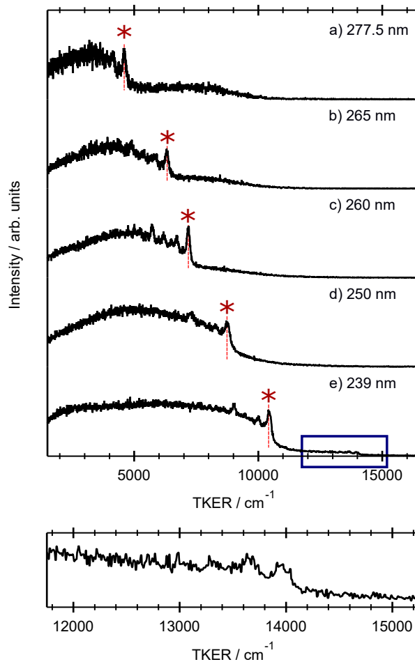
Fig. 4 TKER spectra derived from H atom TOF spectra recorded following photodissociation of 2-thiophenethiol at \lambda_{\text{phot}} = a) 277.5, b) 265, c) 260, d) 250 and e) 239 nm. The peak assigned to \text{H} + \text{R}(\tilde{\text{A}}, v=0) products in each spectrum is indicated by the asterisk. The panel below shows an expanded view of the weak high TKER feature evident in panel (e).
