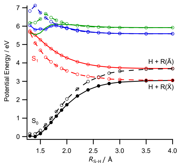
Fig. 5 Unrelaxed PECs along R_{S-H} calculated at the CASPT2(10,8)/cc-pVDZ level for the ground and first three singlet excited states for 2-thiophenethiol with \psi = 80^\circ (filled circles and solid lines) and \psi = 0^\circ (open circles and dashed lines).
