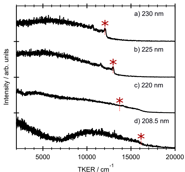
Fig. 6 TKER spectra derived from H atom TOF spectra measured following the photodissociation of 2-thiophenethiol at \lambda_{\text{phot}} = a) 230, b) 225, c) 220 and d) 208.5 nm. The star shows the TKER expected for H + R( \tilde{A} , v=0 ) products at each excitation wavelength.
