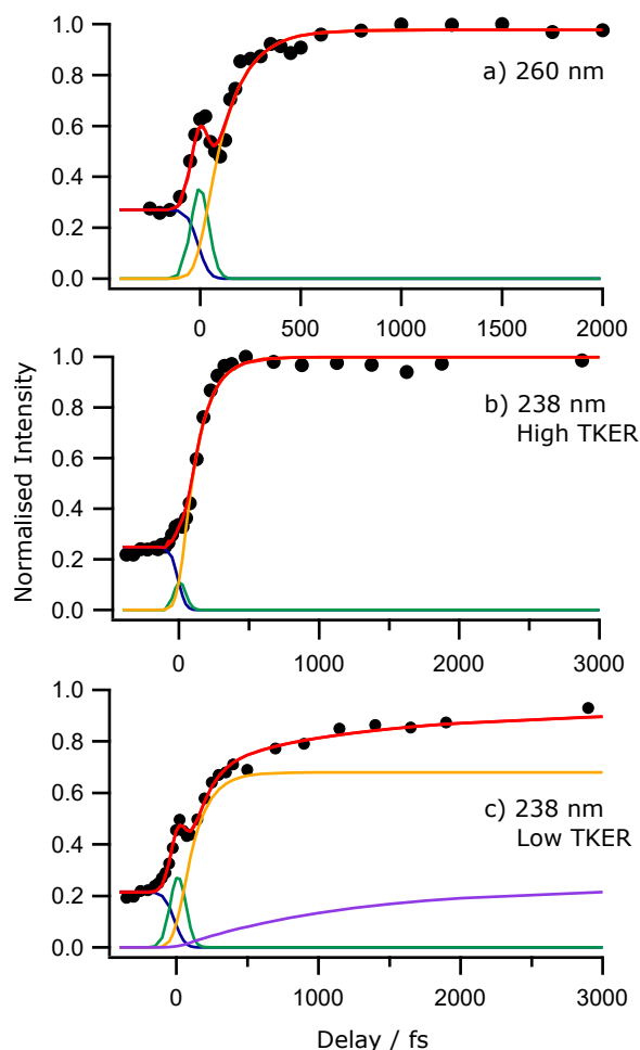
Fig. 8 Normalised H^+ signal transients following excitation of 2-thiophenethiol at 260 nm (a) and 238 nm (b and c). The latter are for signal with TKERs in the range (b) 6000 - 11000 \text{ cm}^{-1} and (c) 0 - 5000 \text{ cm}^{-1} respectively. The filled circles represent the integrated H^+ signal for each TKER of interest and the solid red line represents the overall kinetic fit. Individual fitting components are shown in blue (exponential rise at \Delta t < 0 ), green (exponential decay centred at \Delta t = 0 ) and yellow ( \Delta t > 0 ). The purple line in c) is an additional exponential rise used to fit the long-time increase in intensity.
