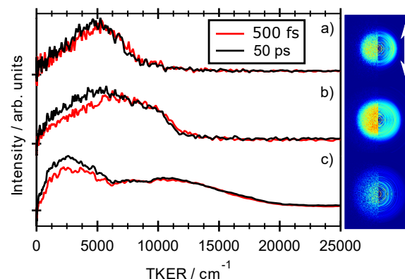
Fig. 7 Raw image and 2-D slice through the reconstructed velocity distribution (left and right half images, respectively) of the H atom fragments resulting from photolysis of 2-thiophenethiol at a) 260, b) 238 and c) 200 nm recorded at \delta t = 500 fs delay time. The double headed arrow indicates the alignment of \epsilon_{\text{phot}} . TKER distributions derived from images recorded at \delta t = 500 fs and 50 ps are shown alongside. Given the poorer signal to noise ratio of the 200 nm image, the TKER spectra in fig. 7(c) have been subjected to a 15-point smoothing prior to display.
