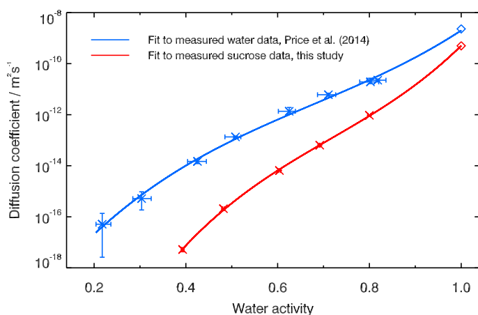
Fig. 5 Measured diffusion coefficients of sucrose and water 59 in aqueous sucrose at 296 K, as a function of water activity. The diffusion coefficients of water and sucrose in water at a water activity of 1.0 are shown using diamonds 63,64 . Solid lines are empirical fits to the data, according to equation 5. Note that error bars are shown for both sets of data but are considerably smaller for the sucrose diffusion coefficients because of the different experimental setup. Uncertainties in water activity are larger for the water diffusion experiments because they incorporate the difference in vapour pressure between normal and heavy water. Since only H 2 O was used for the sucrose diffusion experiments, the error bars are much smaller.
