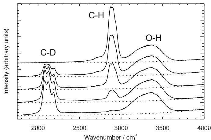
Fig. 2 Raw Raman data for aqueous sucrose showing the gradual decrease in the C-H stretch (at 3100 to 3800 cm -1 ) band and increase in the C-D stretch (at 2000 to 2300 cm -1 ) band as the Raman laser traces a path across the boundary between the deuterated and non-deuterated sucrose droplets. The unchanging band at 3100 to 3600 cm -1 is the O-H stretch. The dotted lines show the Gaussian curve used for the background subtraction.
