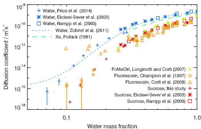
Fig. 9 Diffusion coefficients of water 43,59,65,66 , sucrose 65,66 , fluorescein 39,41 , ferrocene methanol 76 and xenon 25 in aqueous sucrose. Colour corresponds approximately to the size of the diffuser: the largest, sucrose, is shown in red, followed by fluorescein in orange, then ferrocene methanol in yellow-green, xenon in blue-green and finally water, the smallest, shown in blue. Water activities used in this study and reported by Zobrist et al. 43 and Price et al. 59 are converted to water mass fraction using the parameterisation given by Norrish 67 . The grey dashed line represents an extrapolation of the Pollack 25 parameterisation. We include this more speculative regime on the basis that the parameterisation is arrived at via a straight line fit in \log(\text{diffusion coefficient}) vs \log(\text{viscosity}) space; the agreement with the Price et al. 59 water diffusion coefficient data is interesting.
