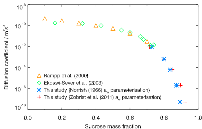
Fig. 6 Diffusion coefficients of sucrose measured using Raman isotope tracer method at 296 K, compared with NMR measurements of sucrose diffusion by Rampp et al. 65 and Ekdawi-Sever et al. 66 . To compare diffusion coefficients on the same scale, water activity was converted to sucrose mass fraction using either the Norrish 67 or the Zobrist et al. 43 parameterisation.
