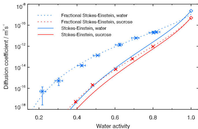
Fig. 7 Measured diffusion coefficients compared with Stokes-Einstein predictions. The diffusion coefficients of water and sucrose in water at a water activity of 1.0 are shown using diamonds 63,64 . The solid lines show the predicted diffusion coefficients of water and sucrose calculated based on the viscosity parameterisation given by Chenlo et al. 69 , using the thermodynamic treatment for water activity of Norrish 67 . The dotted lines show two fractional Stokes-Einstein relationships, i.e. D = C\eta^{-\zeta} where C = 2 \times 10^{-11} and 9 \times 10^{-13} and \zeta = 0.57 and 0.90 for water and sucrose, respectively.
