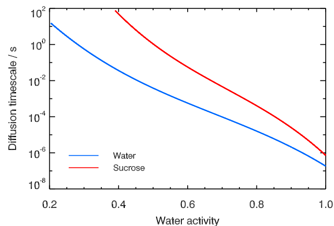
Fig. 10 Diffusion timescales for sucrose and water molecules in aqueous sucrose at 296 K, as a function of water activity, predicted using fits to the diffusion coefficient data and equation 6.
