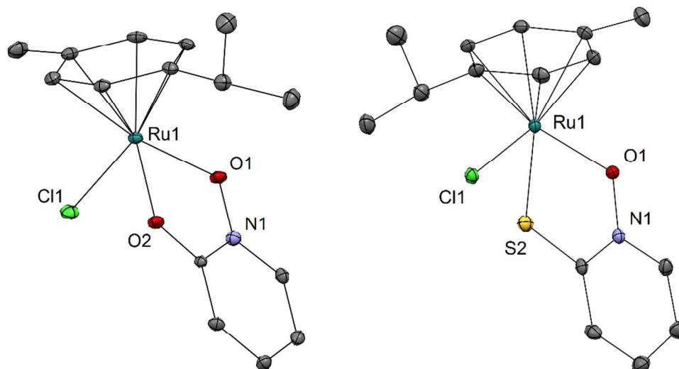
Figure 1: Crystal structures of complexes 1A and 1B with heteroatom labelling. Hydrogen atoms are omitted for clarity of presentation. The ellipsoids are shown at 35% probability level. Selected bond lengths and angles – 1A : Ru1–O1 2.0768(17) Å; Ru1–O2 2.0762(14) Å; Ru1–Cl1 2.4170(6) Å; Ru1–CYM centroid 1.6372(11) Å; O1–Ru1–O2 78.05(6)°; O1–Ru1–Cl1 85.87(5)°; O2–Ru1–Cl1 85.46(5)°; 1B : Ru1–O1 2.0808(18) Å; Ru1–S2 2.3555(7) Å; Ru1–Cl1 2.4487(6) Å; Ru1–CYM centroid 1.6613(12) Å; O1–Ru1–S2 82.73(5)°; O1–Ru1–Cl1 84.53(5)°; S2–Ru1–Cl1 87.34(2)°.
