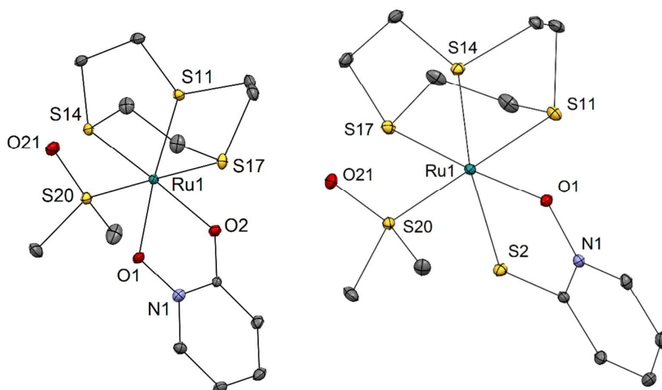
Figure 2: Crystal structures of complexes 2A and 2B with heteroatom labelling. Hydrogen atoms, hexafluorophosphate anions and co-crystallized solvent molecules are omitted for clarity of presentation. The ellipsoids are shown at 35% probability level. Selected bond lengths and angles – 2A : Ru1–O1 2.0786(1) Å; Ru1–O2 2.0974(1) Å; Ru1–S11 2.2913(5) Å; Ru1–S14 2.2888(1) Å; Ru1–S17 2.3421(5) Å; Ru1–S20 2.2596(5) Å; O1–Ru1–O2 79.71(6)°; 2B : Ru1–O1 2.0857(15) Å; Ru1–S2 2.3703(6) Å; Ru1–S11 2.3465(7) Å; Ru1–S14 2.3278(6) Å; Ru1–S17 2.2982(6) Å; Ru1–S20 2.2633(7) Å; O1–Ru1–S2 83.60(4)°.
