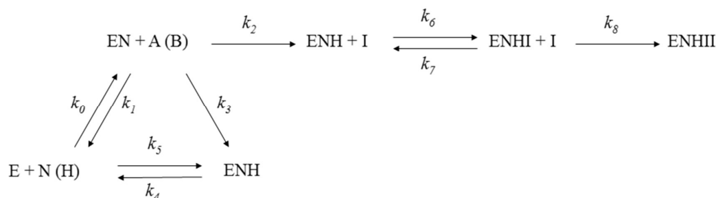
Scheme 2: Universal scheme for inhibition/inactivation of AKR1C enzymes by Ru complexes and ligands. E is free enzyme, N is coenzyme \text{NAD}^+ , EN and ENH are enzyme-coenzyme complexes with oxidized and reduced form of coenzyme, respectively, A, B are the enantiomers of 1-acenaphthenol, and I is inhibitor; k_0 - k_8 are first and second order rate constants.
