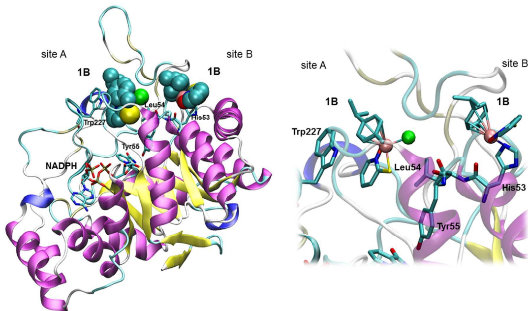
Figure 3: Visualization of 1B binding to AKR1C1 enzyme. Left – complete protein structure with spacefill model of 1B; right – close-up view of the 1B binding site. Binding of Ru complex 1B can be explained by rapid competitive inhibition of the first Ru containing molecule to the holoenzyme ( Site A ), followed by slow substitution of \text{Cl}^- from the complex ( via aqua species ) by a protein nucleophilic side chain in the vicinity of the active site, putatively His53 ( Site B ). Coenzyme NADPH, the catalytic Tyr55, and His53, Leu54 and Trp227 together with two molecules of 1B are depicted.
