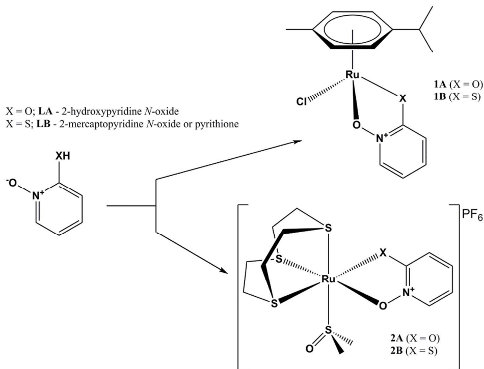
Scheme 1: Reaction path for complexes of series 1 and 2 .
