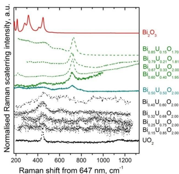
Fig. 5 Raman spectra of the Bi-U-O compositions.
