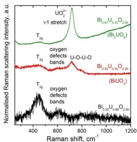
Fig. 6 Raman spectra of \text{Bi}_{0.50}\text{U}_{0.50}\text{O}_{2.00} , \text{Bi}_{0.32}\text{U}_{0.68}\text{O}_{2.00} , and \text{Bi}_{0.67}\text{U}_{0.33}\text{O}_{2.00} .
