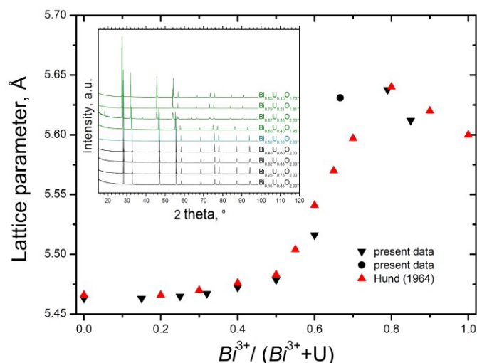
Fig. 1 Lattice parameter variation in the Bi-U-O system as a function of the substitution degree. For \text{Bi}_{0.67}\text{U}_{0.33}\text{O}_{2.00} (●), see discussions. Inset: XRD patterns of the different mixed oxides analysed in this study.
