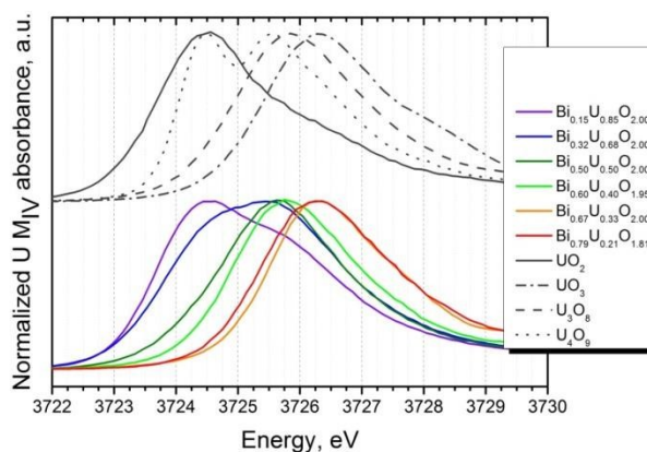
Fig. 3 U M_{IV} XANES spectra of Bi-U-O compositions.
