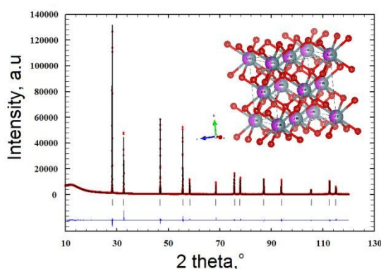
Fig. 7 Rietveld refinement of \text{BiUO}_4 . Comparison between the observed (Yobs, in red) and calculated (Ycalc, in black) X-ray diffraction pattern of \text{BiUO}_4 phase. Yobs-Ycalc (in blue) is the difference between the experimental and calculated intensities. The Bragg reflections are marked in black ticks.
