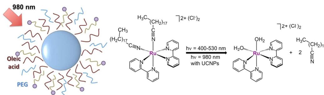
Fig. 5. Schematic representation of the NIR-light activation of the prodrug candidate [\text{Ru}(\text{bpy})_2(\text{C}_{18}\text{H}_{37}\text{CN})_2][\text{Cl}]_2 (*) mediated by UCNPs. Adapted from references 30.
