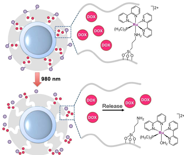
Fig. 6. Schematic representation of the nanocarrier developed by Wu and coworkers. Doxorubicin (DOX, \bullet ) is release by NIR-light activation of a Ru polypyridyl complex ( \bullet ) acting as valve. The figure is adapted from reference 31
