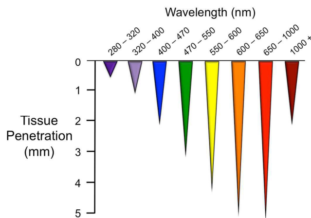
Fig. 1. Penetration depth of light of different wavelengths in skin tissue. Image adapted from reference 1.
