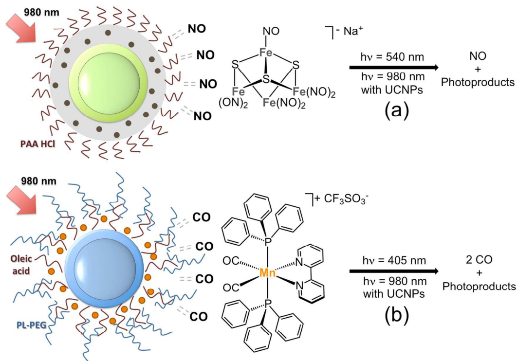
Fig. 3. Schematic representation of UCNPs nanocarriers for the NIR-light photorelease of (a) NO from RBS (•) and (b) CO from the complex cis,trans -[Mn(bpy)(CO) 2 (PPh 3 ) 2 ][CF 3 SO 3 ] (•). Adapted from references 15 and 18.
