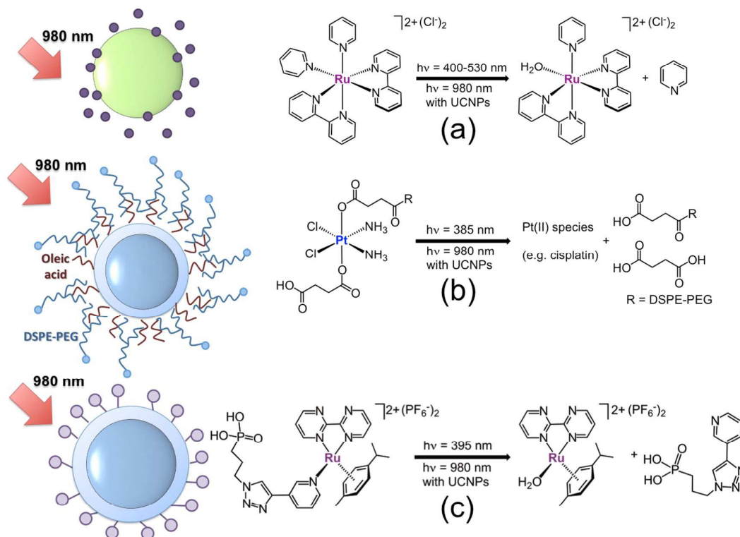
Fig. 4. Schematic representation of UCNP systems for the NIR-light activation of (a) cis -[Ru(bpy) 2 (py) 2 ][Cl] 2 (•), (b) cis,cis,trans -[Pt(NH 3 ) 2 Cl] 2 (O 2 CCH 2 CH 2 CO 2 H) 2 functionalized with DSPE-PEG (•) and (c) [(η 6 -p-cym)Ru(bpm)(P-Trz-Py)][PF 6 ] 2 (•). Adapted from references 20, 26 and 28.
