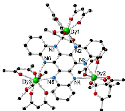
Fig. 1 Molecular structure of 1 . For clarity, the methyl groups on the [\text{thd}]^- ligands and the hydrogen atoms are not shown.
