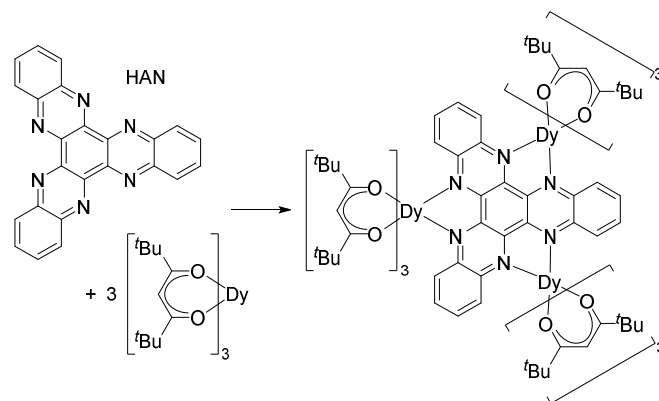
Scheme 1. Synthesis of [\{(thd)_3Dy\}_3HAN] ( 1 ).
