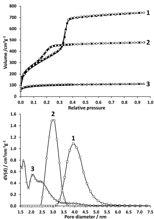
Fig. 5 Top: Nitrogen adsorption (filled symbols) and desorption (open symbols) isotherms of ASNCs after extraction with thermal pretreatment (1), calcination (2), and extraction without thermal pretreatment (3). Bottom: Respective pore size distributions.
