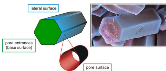
Fig. 1 Illustration of the different surface regions of ASNCs. The particle shown in the scanning electron microscopy image has a length of approximately 5 \mu\text{m} . The average pore (nanochannel) diameter is typically in the range of 2.5 to 4 nm.
