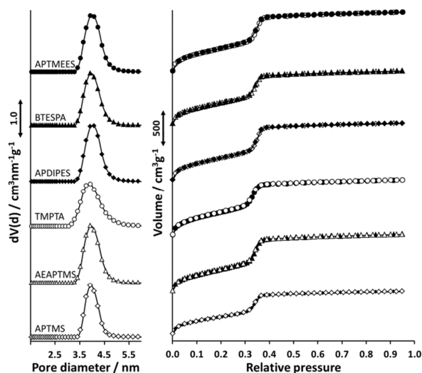
Fig. 6 Left: Pore size distributions of amino-functionalized ASNCs prepared by post-condensation and subsequent extraction of the SDA. The abbreviations indicate the respective NH-silane used in the post-condensation (NH-silane/TEOS = 0.1). Right: Corresponding nitrogen sorption isotherms.
