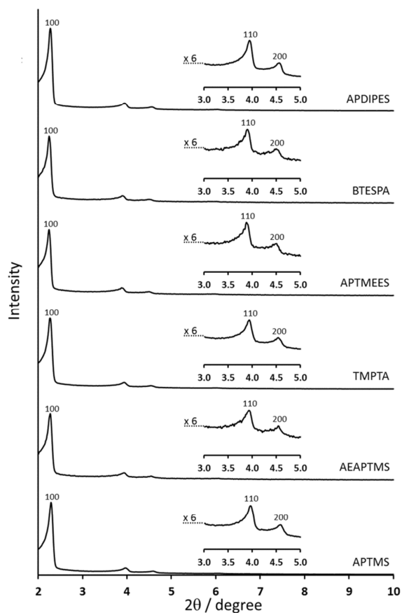
Fig. 8 XRD patterns of amino-functionalized ASNCs prepared by post-condensation and subsequent extraction of the SDA. The abbreviations indicate the respective NH-silane used in the post-condensation (NH-silane/TEOS = 0.1).
