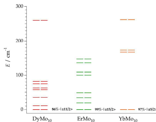
Fig. 8 Energy level scheme and main contributions to the ground state wave function for DyMo_{10} , ErMo_{10} and YbMo_{10} .
