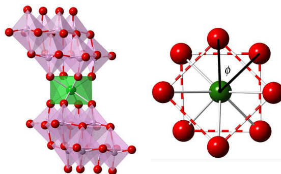
Fig. 1 (left) Polyhedral and ball-and-stick representation of \text{LnMo}_{16} series and (right) projection of the coordination sphere showing the square antiprismatic coordination site.
