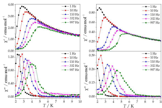
Fig. 7 In-phase (up) and out-of-phase (down) dynamic susceptibility of DyMo_{10} (left) and YbMo_{10} (right) under an applied field of 1000 Oe. The frequencies are shown in the legend. Solid lines are eye-guides.
