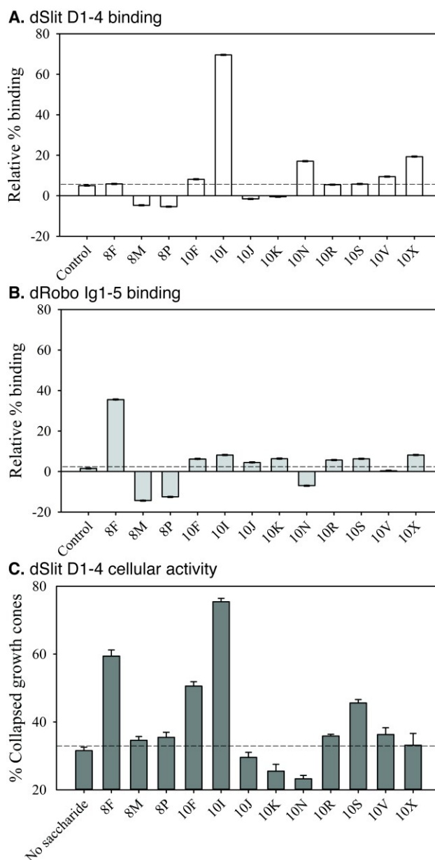
Figure 6. PMHS saccharides possess differential abilities to bind dSlit D1-4 or dRobo Ig1-5-Fc and promote dSlit D1-4 cellular activity. PMHS ~ 8-mer and ~10-mer SAX-HPLC fractions were screened for binding to (A) his 6 -cmyc-dSlit D1-4 and (B) dRobo Ig1-5-IgG1Fc fusion protein using a competition ELISA. % binding values shown represent means of triplicate wells containing competitor relative to means of triplicate wells lacking competitor and error bars represent the % combined standard deviation calculated as described in Experimental Procedures. Control represents protein binding to a surface lacking immobilised biotinylated heparin saccharides. Data are representative of four separate experiments. Fractions were also screened for their ability to rescue (C) His 6 -cmyc-dSlit D1-4 ex vivo chick retinal axon growth cone collapse following treatment with heparinases I-III. Collapsed and uncollapsed growth cones were counted in blind conditions across several pieces of retina for ~100 growth cones and the % of collapsed growth cones calculated. Values shown are the mean % of collapsed growth cones calculated from three groups of retinal pieces and error bars represent the standard deviation for % values. Data are representative of two separate experiments.
