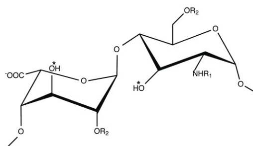
Figure 1. Schematic of the structure of heparin/HS disaccharide repeats. Depicted are \alpha -L-iduronate and \alpha -D-glucosamine. R_1 = H , acetyl or SO_3^- and R_2 = H or SO_3^- . \alpha -L-iduronic acid is formed from \beta -D-glucuronic through epimerization of the carboxyl group. * indicates sites where there is a major increase in sulfation during oversulfation of heparin.
