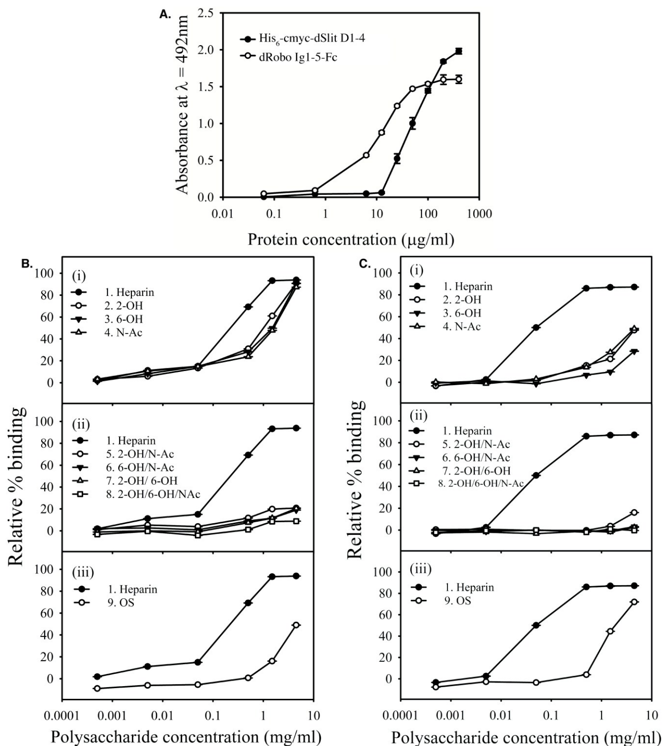
Figure 3. dSlit D1-4 and dRobo Ig1-5-Fc interact differently with heparin and chemically-modified heparins. (A) Binding of different concentrations of \text{His}_6\text{-cmyc-dSlit D1-4} and \text{dRobo Ig1-5-Fc} to a nitrous acid generated heparin 10-mer SEC fraction, surface-immobilised through biotinylation and streptavidin capture. Binding was determined using an ELISA and absorbance values shown are the mean of triplicates and error bars represent the standard deviation. Data are representative of three separate experiments. Binding of (B) \text{His}_6\text{-cmyc-dSlit D1-4} and (C) \text{dRobo Ig1-5-Fc} fusion protein to varying concentrations of soluble chemically-modified heparins (Table 1) determined by inhibition of protein binding to an immobilized \sim 10 -mer heparin saccharide fraction using a competition ELISA. (i) Compound 1 (heparin), 2 (2-OH), 3 (6-OH), 4 (N-Ac), (ii) Compound 1 (heparin), 5 (2-OH/N-Ac), 6 (6-OH/N-Ac), 7 (2-OH/6-OH), 8 (2-OH/6-OH/N-Ac) and (iii) Compound 1 (heparin) and 9 (OS). % binding values shown represent means of triplicate wells containing competitor relative to means of triplicate wells lacking competitor and error bars represent the % combined standard deviation. All calculations were performed as described in Experimental Procedures. Data are representative of four separate experiments.
