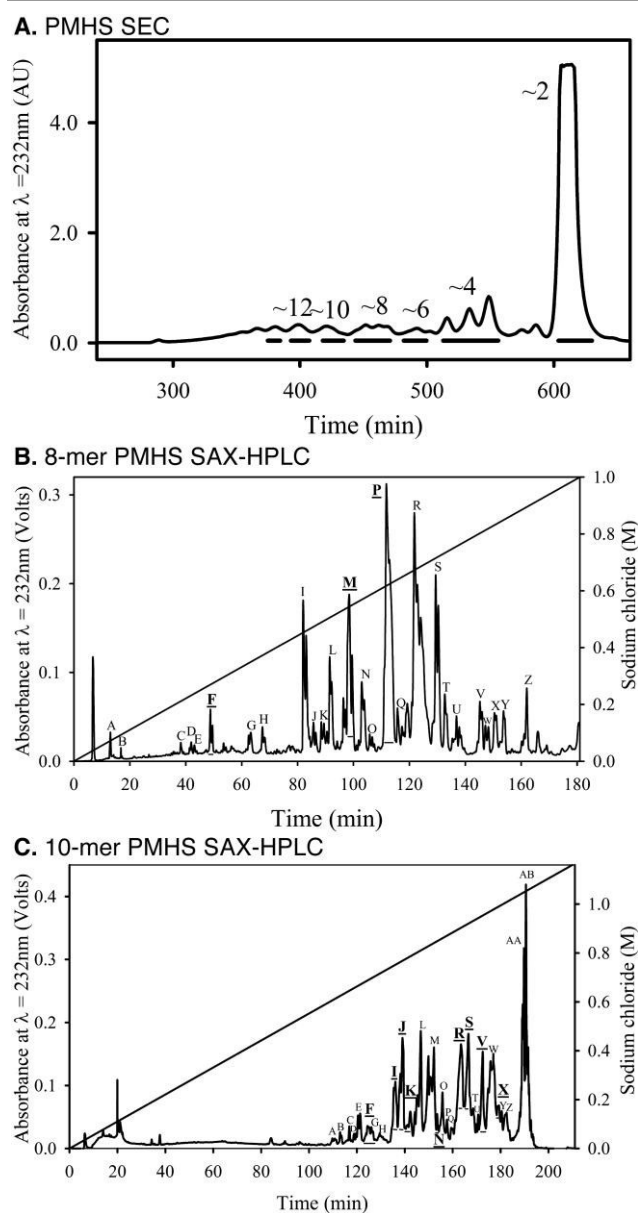
Figure 5. Generation of saccharide chromatographic fractions. PMHS was partially digested with heparinase III and saccharide mixtures separated by (A) SEC. Fractions from SEC that contain (B) ~ 8-mer and (C) ~ 10-mer saccharides were then further separated by SAX-HPLC. Fractions across selected peaks were broadly estimated to contain HS/heparin oligosaccharides displaying increasing degrees of polymerization (shown by even integers). Pooling is shown by horizontal lines beneath peaks. SAX sub-fractions in underlined bold correspond to those used in assays. Chromatography elution profiles were reproducible across multiple runs.
