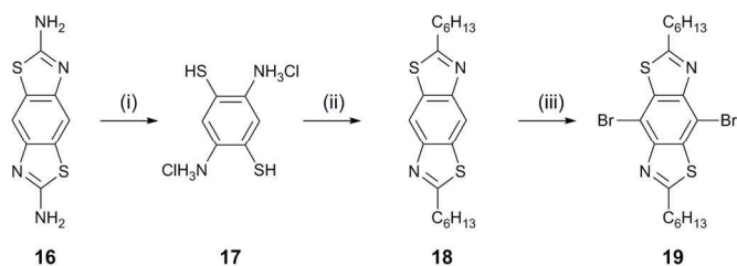
Scheme 1. Reagents and conditions: (i) KOH reflux, then HCl; (ii) heptanoyl chloride, trimethylsilyl polyphosphate, 1,2-dichlorobenzene, reflux; (iii) bromine, dichloromethane, 0°C.
