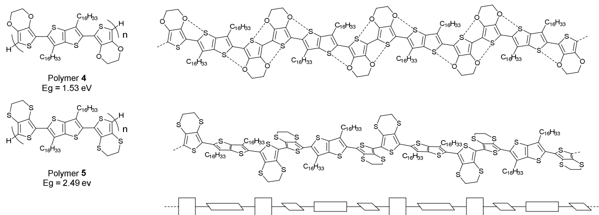
Figure 3. Structures of polymers 4 and 5 with the twisted conformation of 5 in schematic form shown on the bottom.
