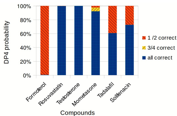
Fig. 3 Overall DP4 probabilities assigned to drug compound diastereomers using MacroModel and NWChem. Only diastereomers with probabilities greater than 0.1% shown.
