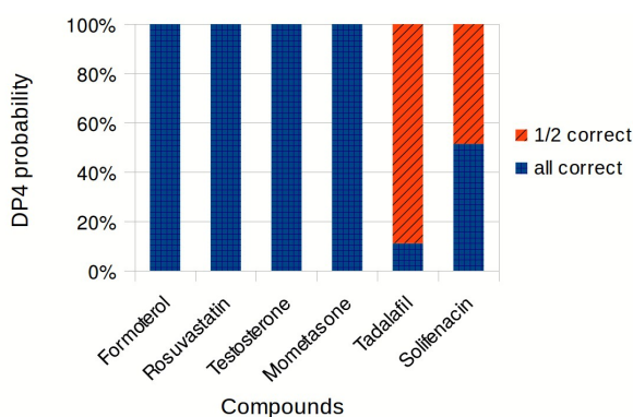
Fig. 5 Overall DP4 probabilities assigned to drug compound diastereomers using Tinker and NWChem. Only diastereomers with probabilities greater than 0.1% shown.
