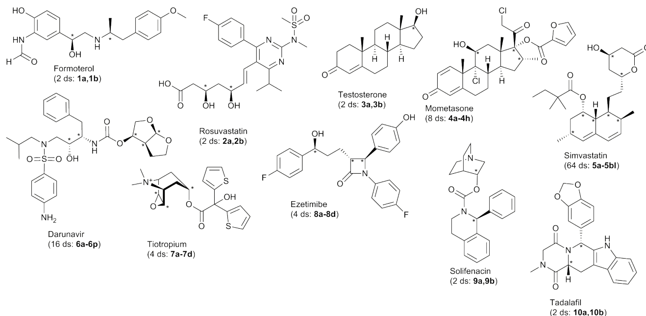
Fig. 1 Stereochemically rich drug molecules selected for DP4 study. Diastereomer count shown. Diastereomers labelled with letters a-bl, a being the correct diastereomer. Configuration was varied at chiral centres marked with '*'.
