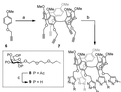
Scheme 2. Synthesis of a galactosylated pentavalent pillar[5]arene-based glycocluster using a penta-propargylated core scaffold. Reagents and conditions: (a) paraformaldehyde, BF 3 •OEt 2 , Cl(CH 2 ) 2 Cl, r.t., 50%; (b) 1-azido-3,6-dioxa-octyl 2,3,4,6-tetra- O -acetyl-β-D-galactopyranoside, CuSO 4 , sodium ascorbate, DMF, 110°C, 15 min, μwaves, 76%; (c) MeOH, Et 3 N, H 2 O, r.t., 16 h, >95%.
