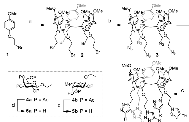
35 Scheme 1. Synthesis of pentavalent pillar[5]arene-based glycoclusters using a penta-azido core scaffold. Reagents and conditions: (a) paraformaldehyde, BF 3 •OEt 2 , Cl(CH 2 ) 2 Cl, r.t., 84%; (b) NaN 3 , DMF, 100°C, 12 h, 91%; (c) propargyl 2,3,4,6-tetra- O -acetyl-β-D-galactopyranoside or propargyl 2,3,4-tri- O -acetyl-α-D-fucopyranoside, 40 CuI, i Pr 2 NEt, DMF, 110°C, 15 min, μwaves, 87% ( 4a ), 93% ( 4b ); (d) MeOH, Et 3 N, H 2 O, r.t., 16 h, >95% ( 5a and 5b ).
