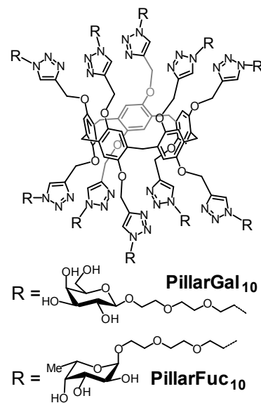
Figure 3. Structures of the galactosylated ( PillarGal 10 ) and fucosylated ( PillarFuc 10 ) decavalent pillar[5]arene-based glycoclusters.
