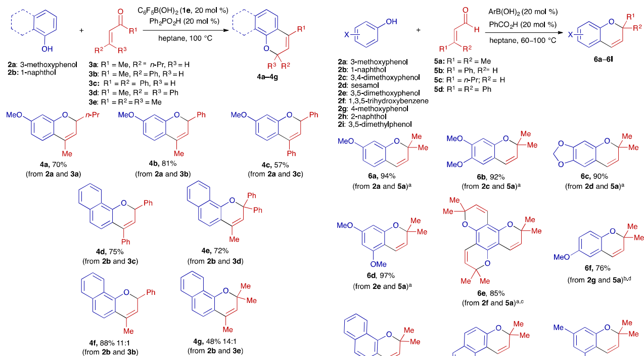
Scheme 2 Condensations of \alpha,\beta -unsaturated ketones with phenol derivatives. Reaction conditions: phenol (0.2 mmol), enone (0.4 mmol), 1e (20 mol %), Ph 2 PO 2 H (20 mol %) in heptane (1 mL) at 100 °C for 3 h under argon. Isolated yields after purification by chromatography on silica gel are listed. Products 4f and 4g were obtained as mixtures of endocyclic and exocyclic olefin isomers.
