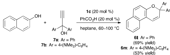
Scheme 5 Synthesis of naphthopyrans from propargylic alcohols.
