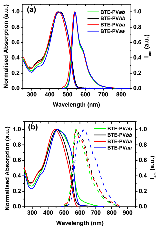
Fig. 1 Normalized absorption (solid) and emission (dash) spectra of the polymers (a) in dilute chloroform solutions and (b) of the polymer films.
