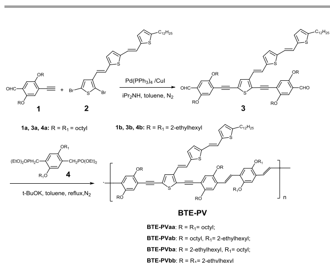
Scheme 1. Synthesis of monomers ( 3a , 3b ) and of conjugated polymers BTE-PVs.
