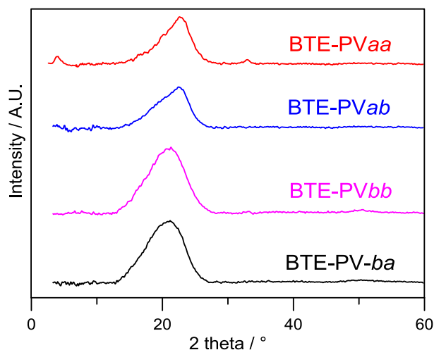
Fig. 3 XRD patterns of polymer films drop-caste onto zero-background quartz substrate.
