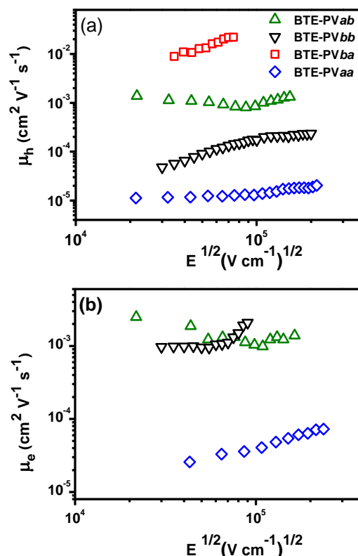
Fig. 2 Hole mobility (a) and electron mobility (b) as a function of the square root of the electric field for: BTE-PVaa (blue diamonds); BTE-PVab (green triangles); BTE-PVba (red squares); BTE-PVbb (inverted triangles).
